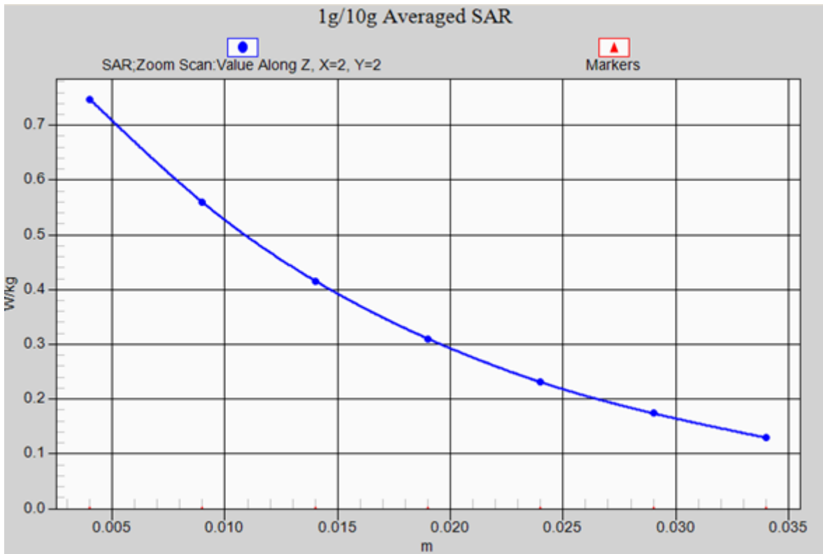
GSM 850/Back side Low-axis scan
