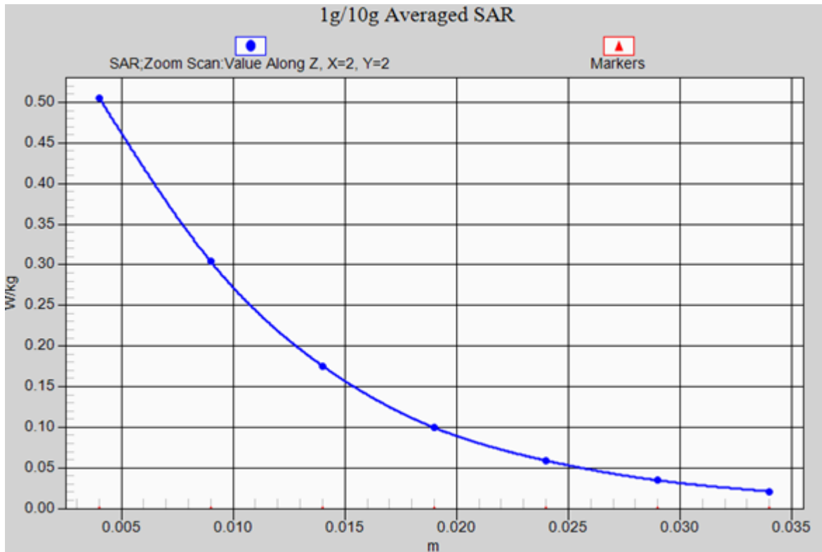
GSM 1900/Back side High-axis scan
