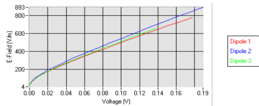
Calibration curves
