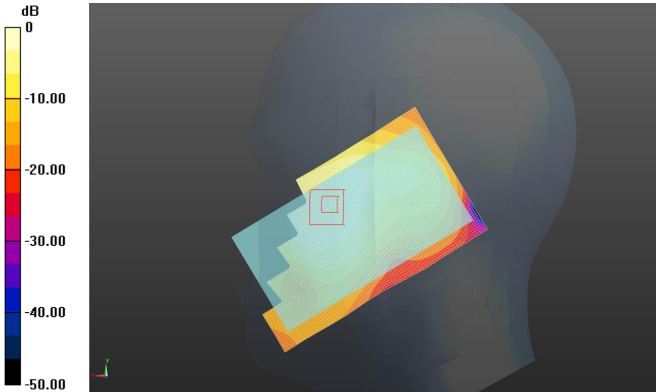
Left Head Cheek (PCS1900 Middle Channel)
