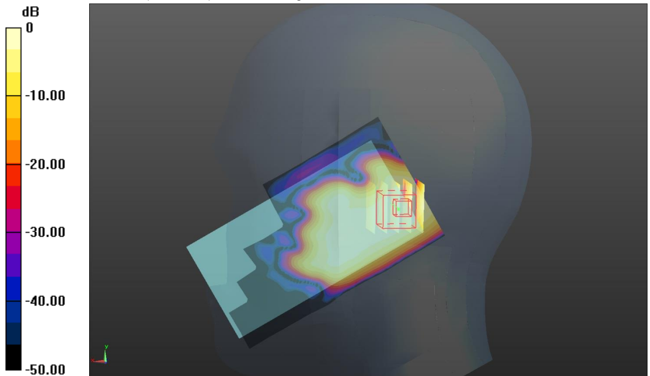
Left Head Cheek (WLAN middle Channel)
