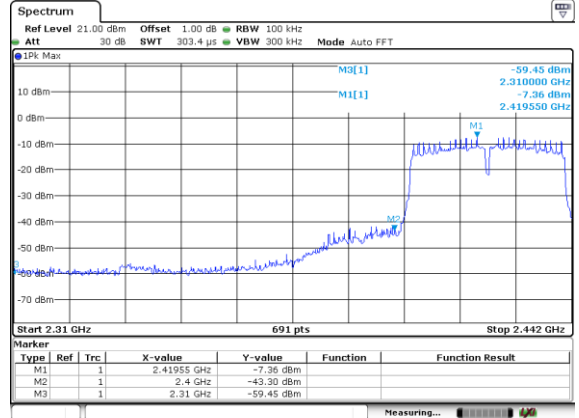
CH03-Bandedge
