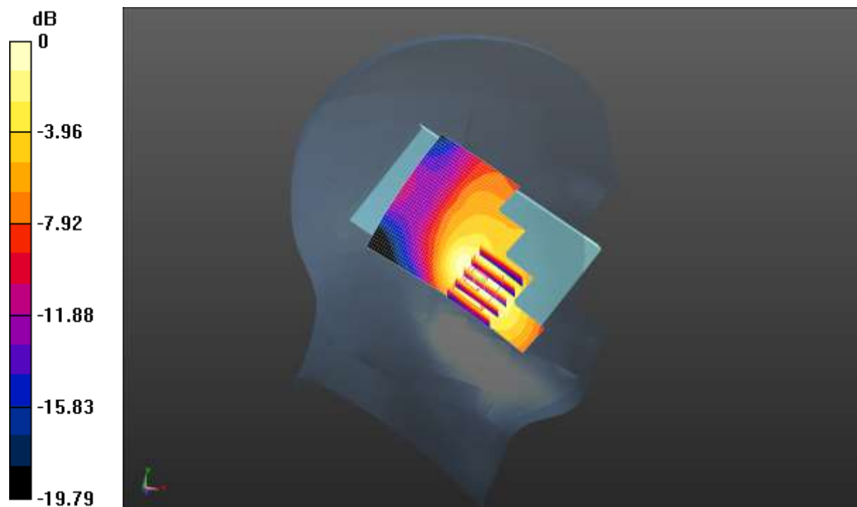
0 dB = 0.276 W/kg = -5.59 dBW/kg
