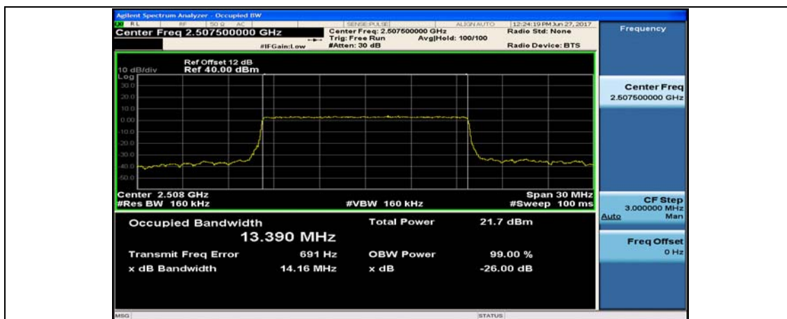
Band7_15MHz_16QAM_20825_75RB#0
