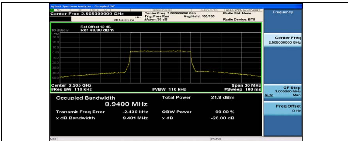
Band7_10MHz_16QAM_20800_50RB#0
