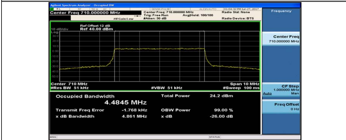
Band17_5MHz_16QAM_23790_25RB#0
