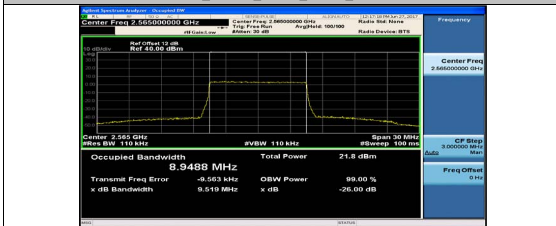
Band7_10MHz_16QAM_21400_50RB#0
