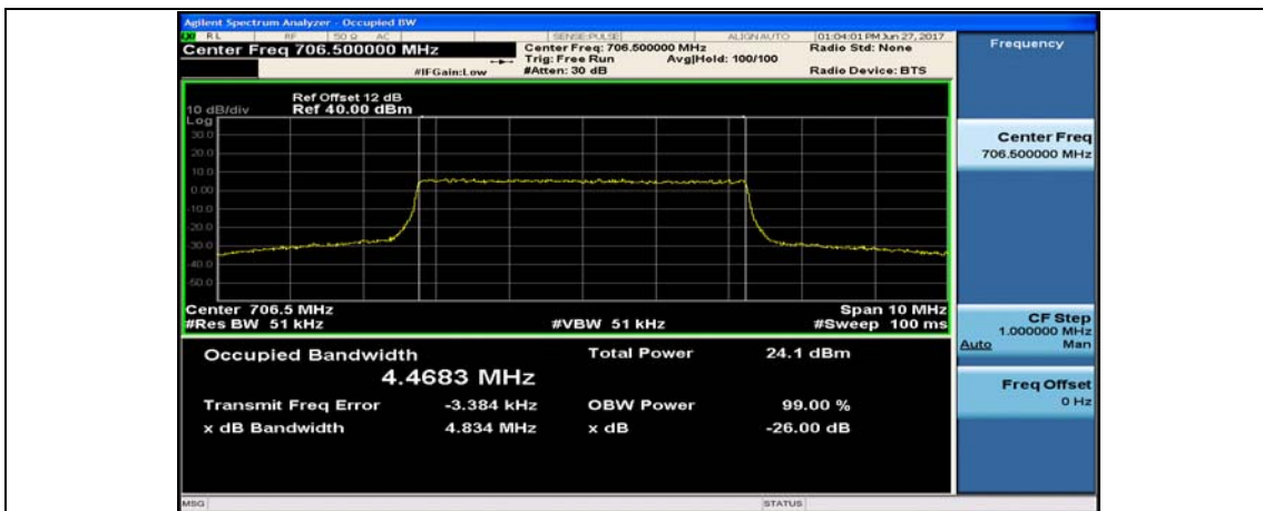
Band17_5MHz_16QAM_23755_25RB#0
