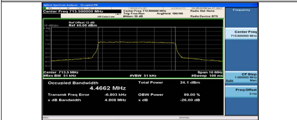
Band17_5MHz_16QAM_23825_25RB#0
