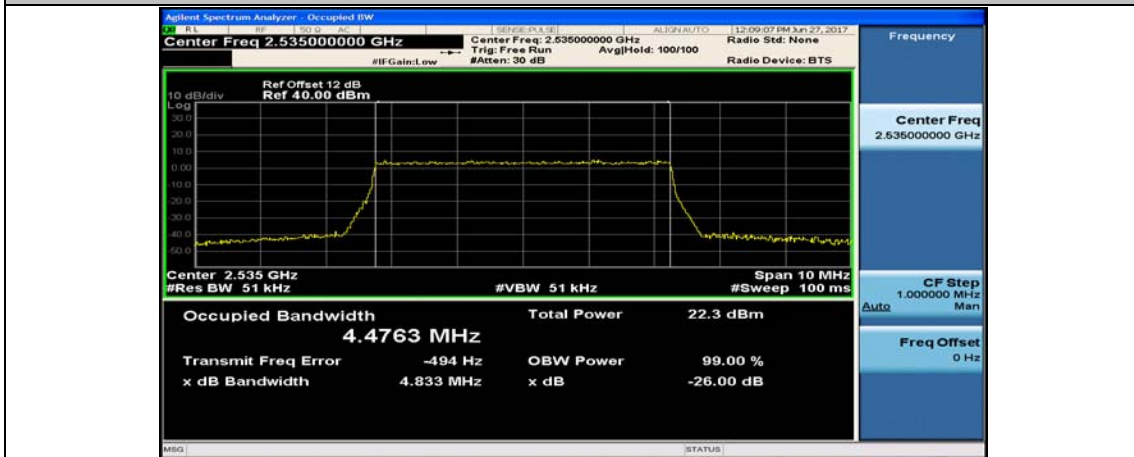
Band7_5MHz_16QAM_21100_25RB#0
