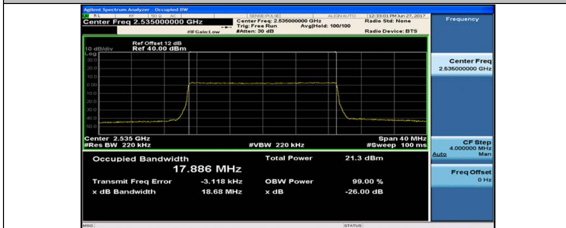
Band7_20MHz_16QAM_21100_100RB#0
