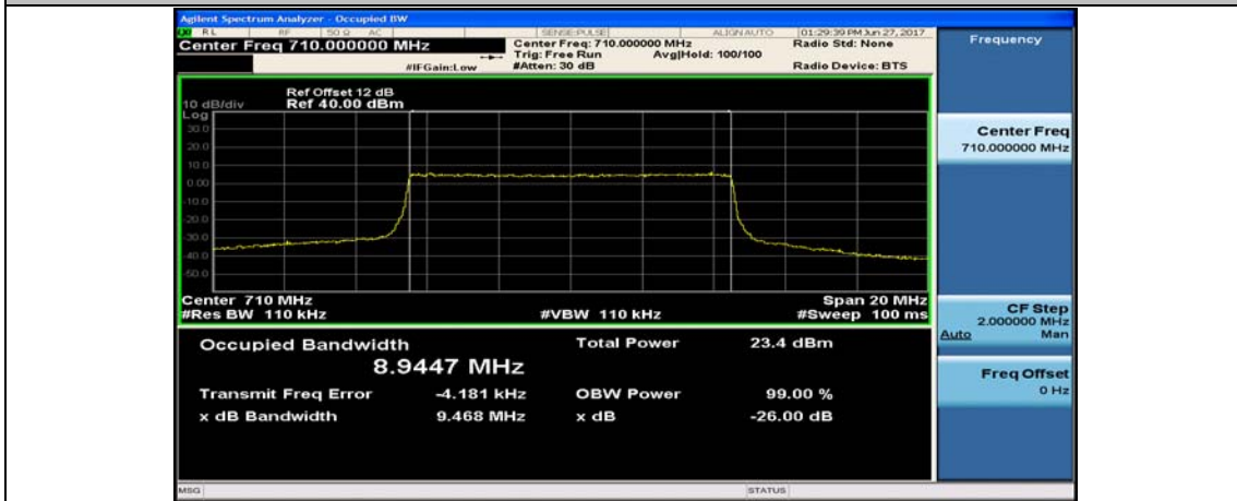
Band17_10MHz_16QAM_23790_50RB#0
