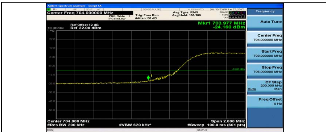
Band17_10MHz_QPSK_23800_50RB#0
