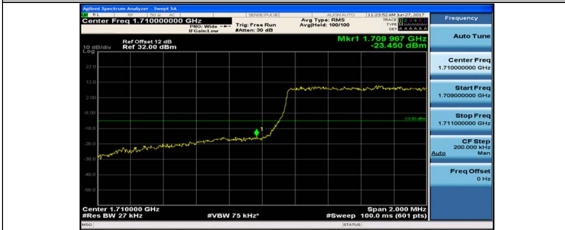
Band4_1.4MHz_QPSK_20393_6RB#0
