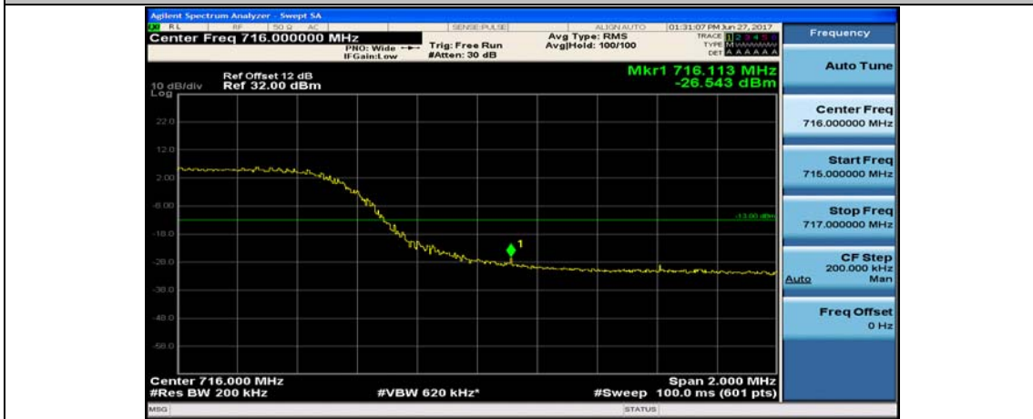
Band17_10MHz_16QAM_23800_50RB#0
