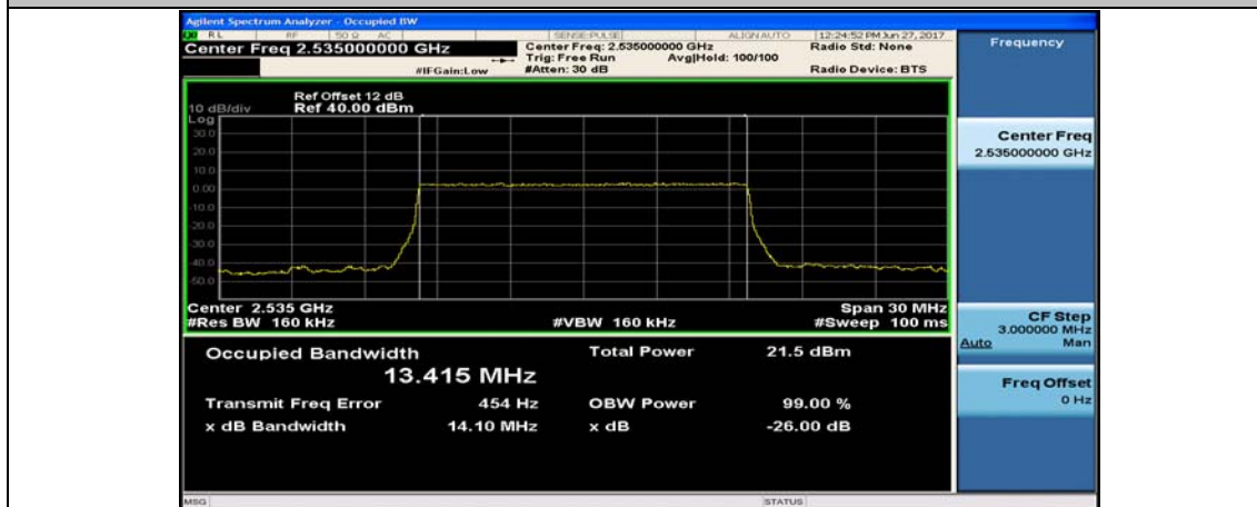
Band7_15MHz_16QAM_21100_75RB#0
