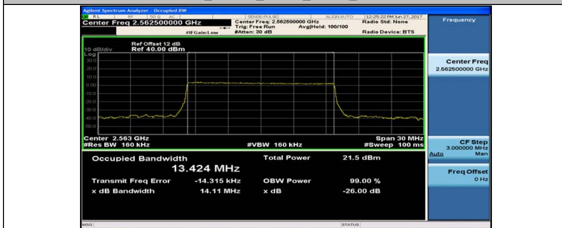
Band7_15MHz_16QAM_21375_75RB#0
