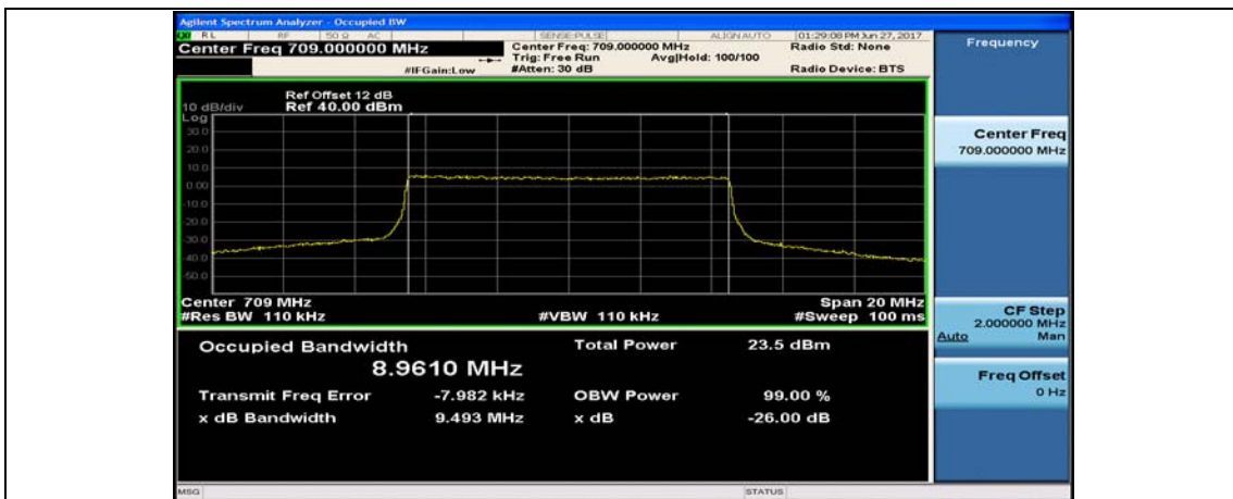
Band17_10MHz_16QAM_23780_50RB#0
