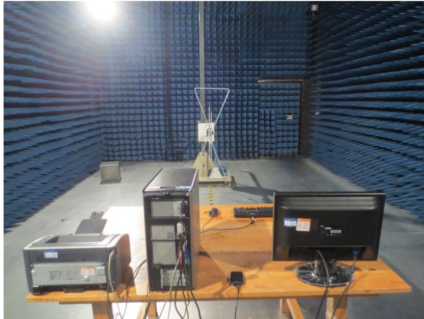
Radiated Emission
