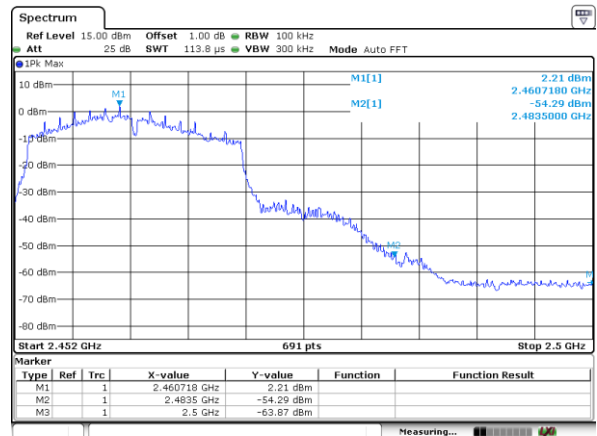
CH11-Bandedge
