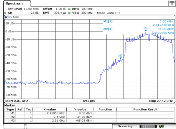
CH03-Bandedge
