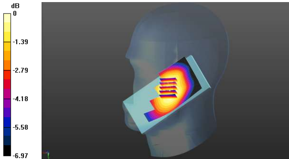
0 dB = 0.0524 W/kg = -12.81 dBW/kg
