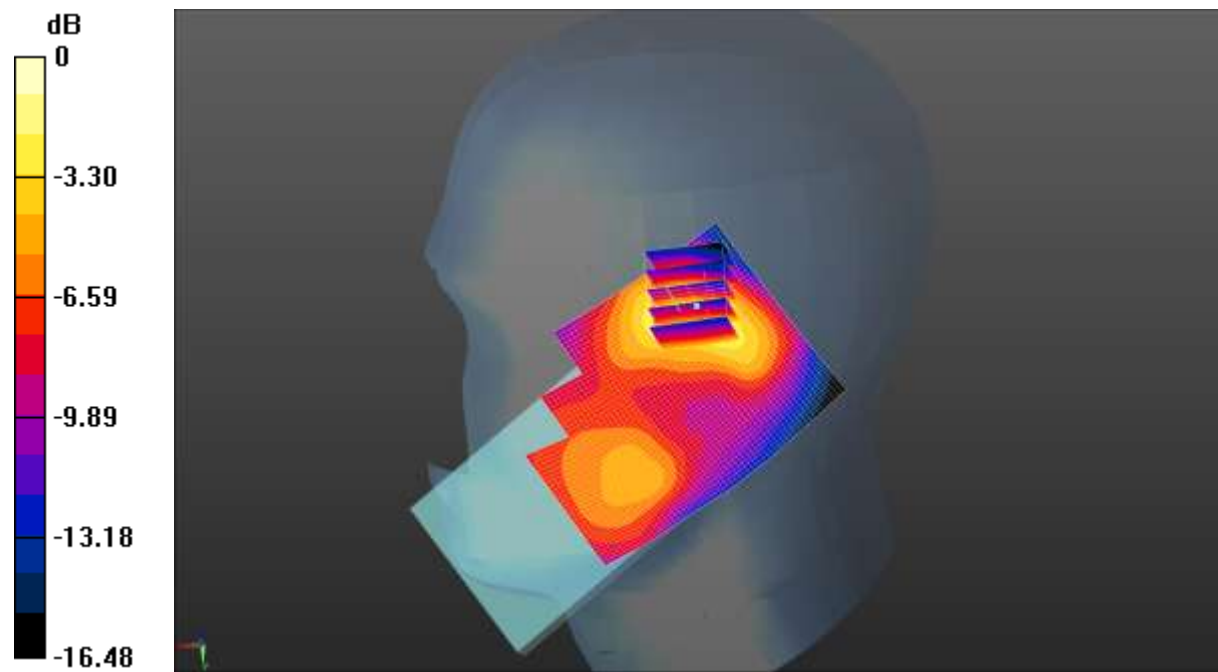
0 dB = 0.221 W/kg = -6.56 dBW/kg
