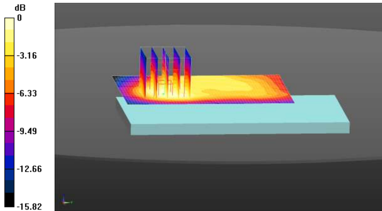
0 dB = 0.489 W/kg = -3.11 dBW/kg
