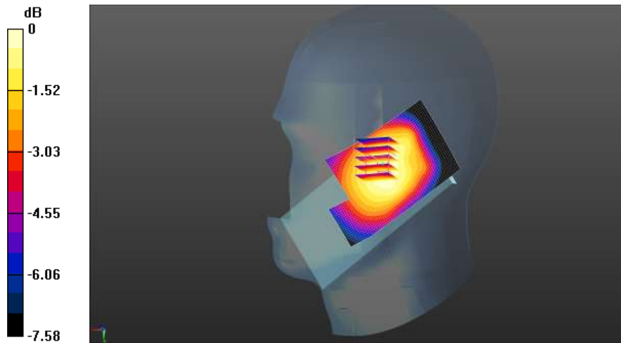
0 dB = 0.0347 W/kg = -14.60 dBW/kg
