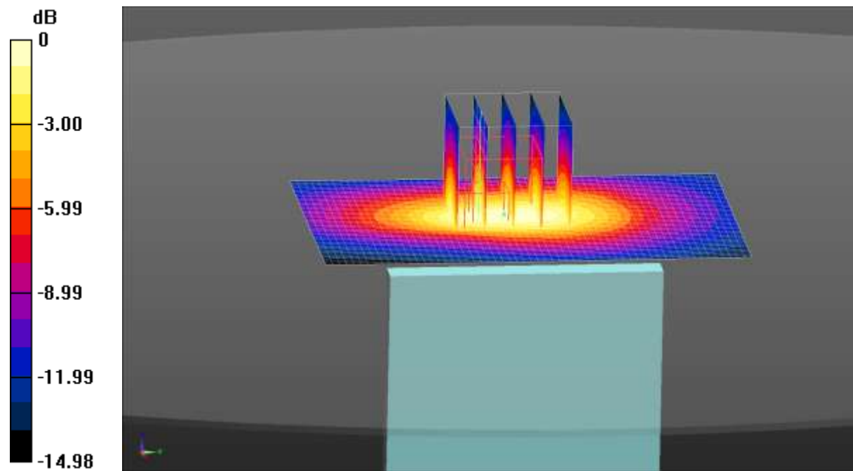
0 dB = 0.518 W/kg = -2.86 dBW/kg
