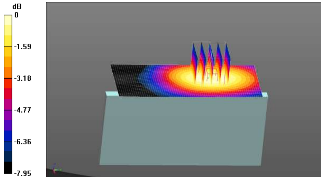
0 dB = 0.0318 W/kg = -14.98 dBW/kg
