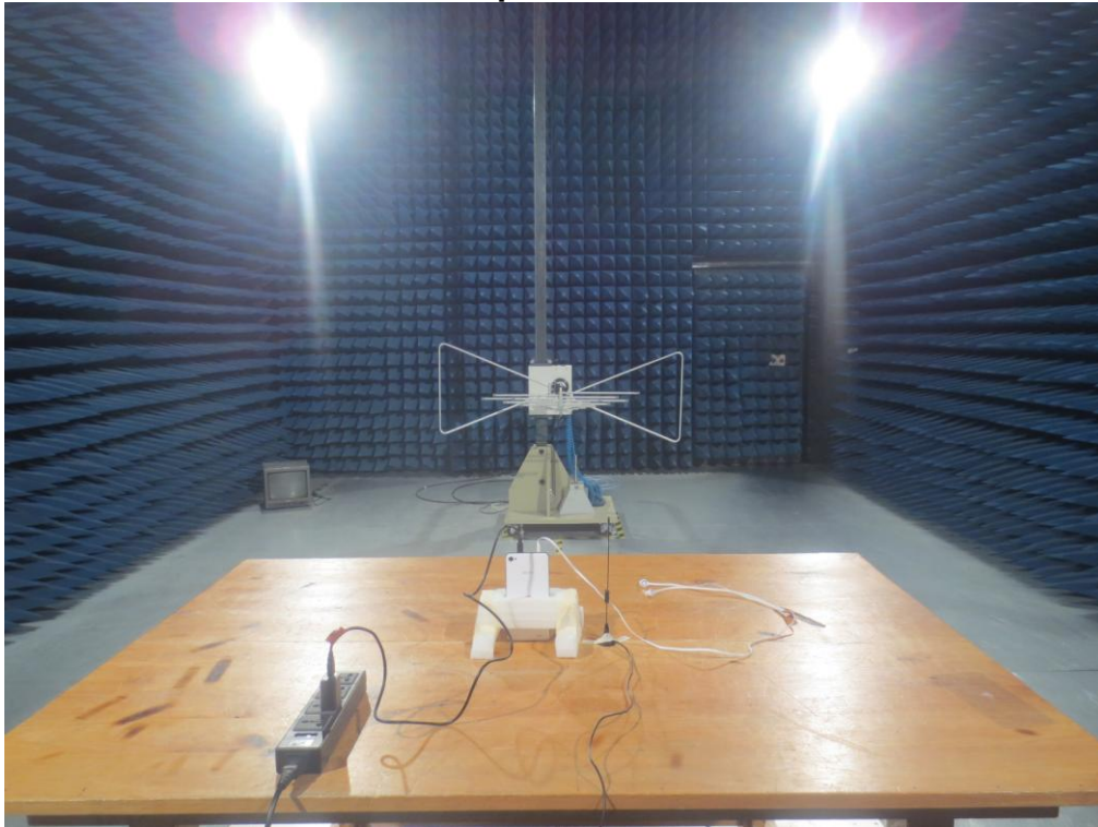
Model No.: A55GL Radiated Spurious Emission
