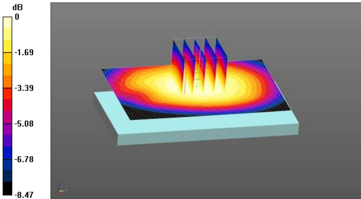
0 dB = 0.760 W/kg = -1.19 dBW/kg
