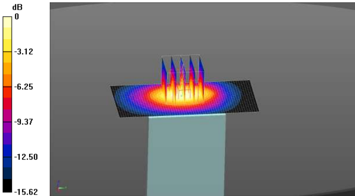
0 dB = 0.495 W/kg = -3.05 dBW/kg
