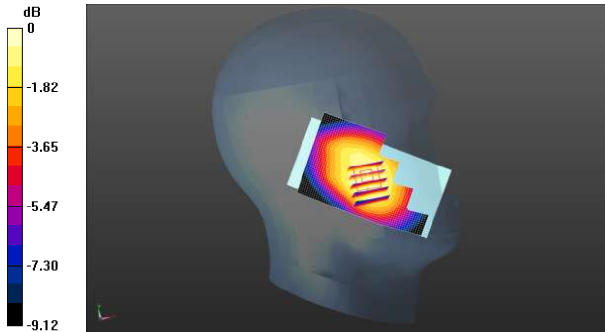
0 dB = 0.464 W/kg = -3.33 dBW/kg
