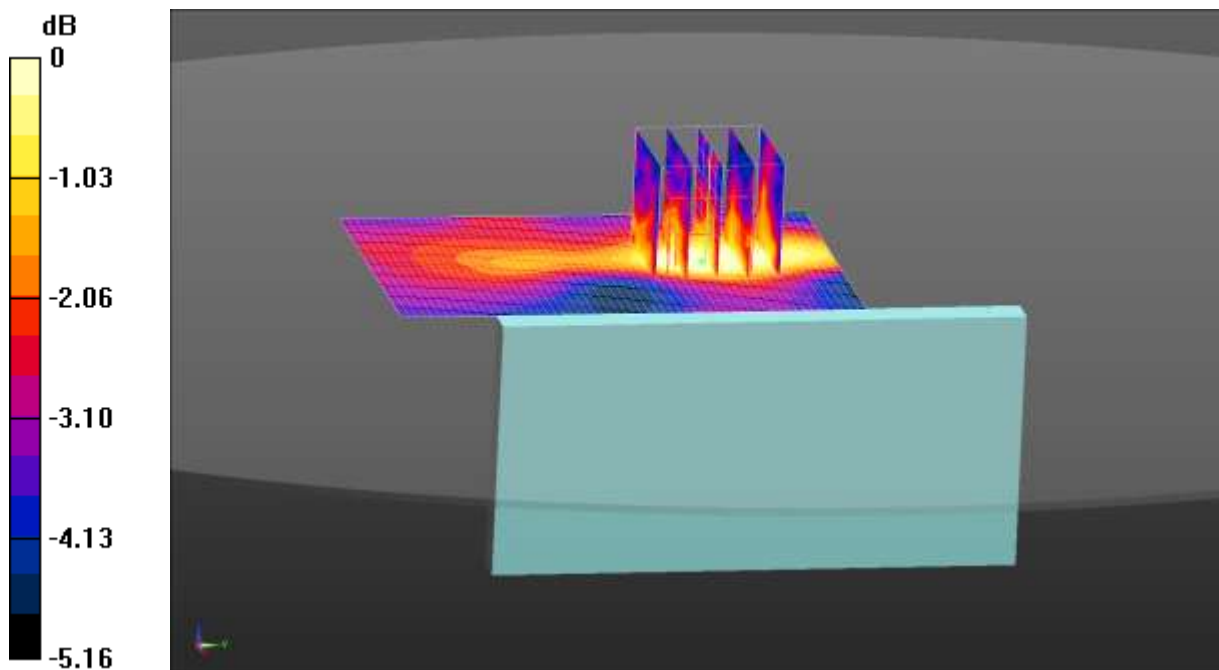
0 dB = 0.0169 W/kg = -17.72 dBW/kg
