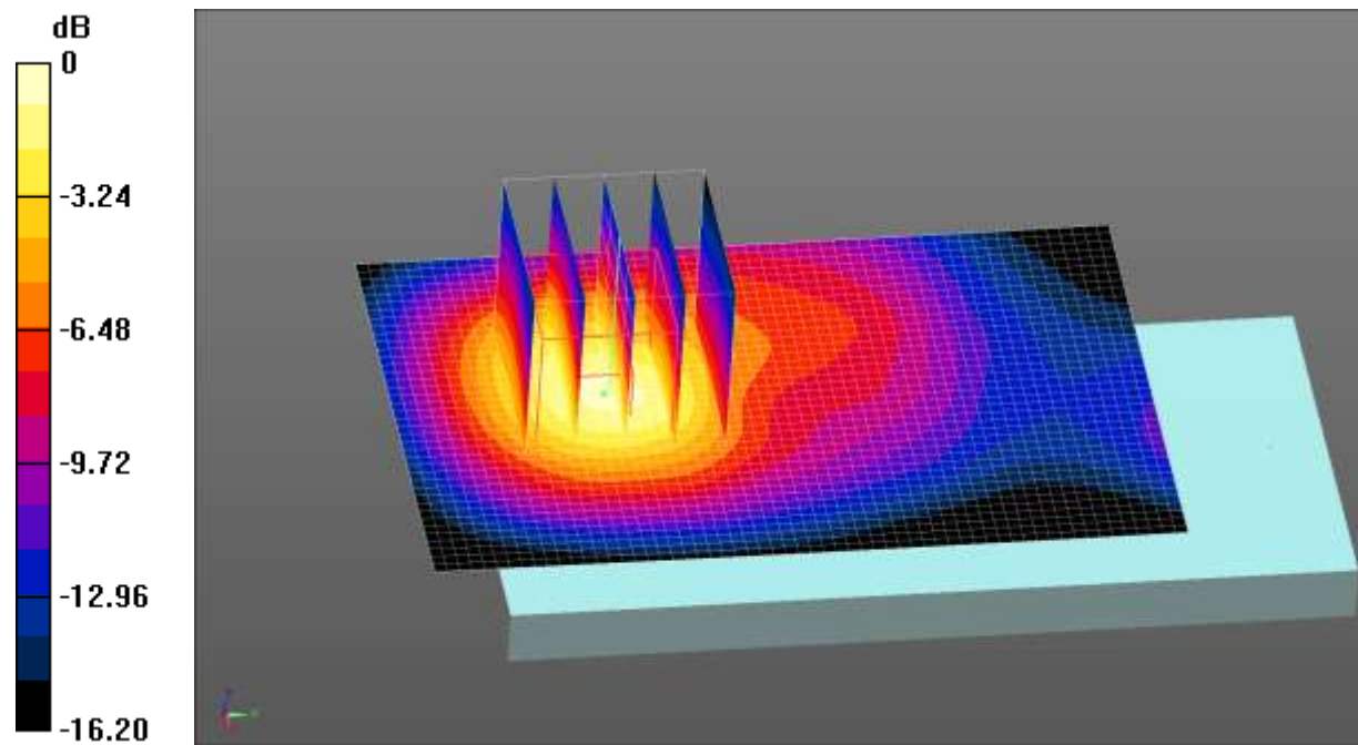
0 dB = 0.585 W/kg = -2.33 dBW/kg
