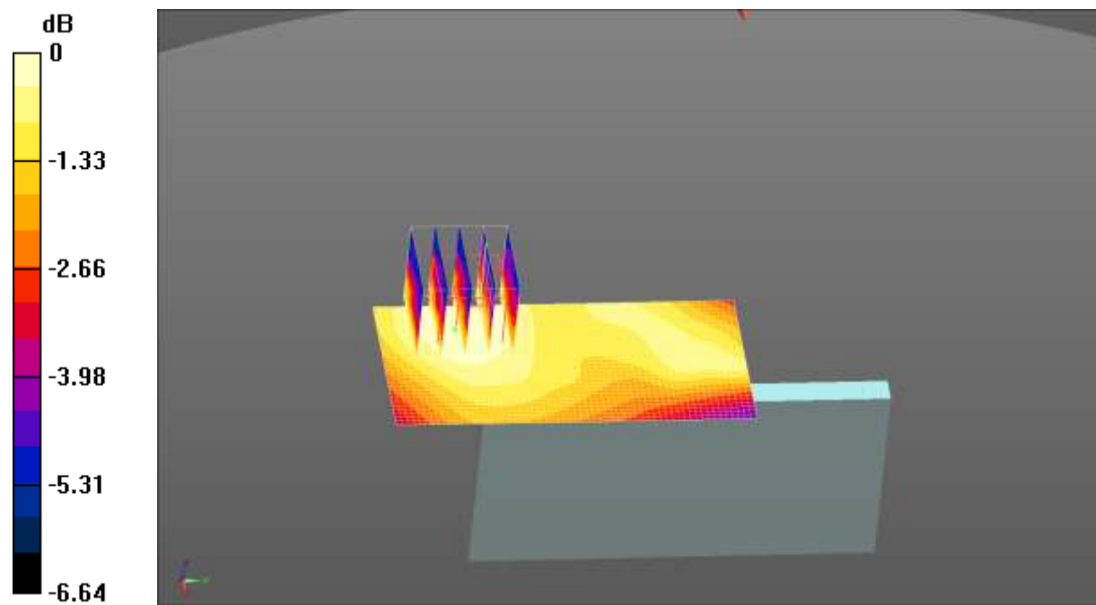
0 dB = 0.0250 W/kg = -16.02 dBW/kg
