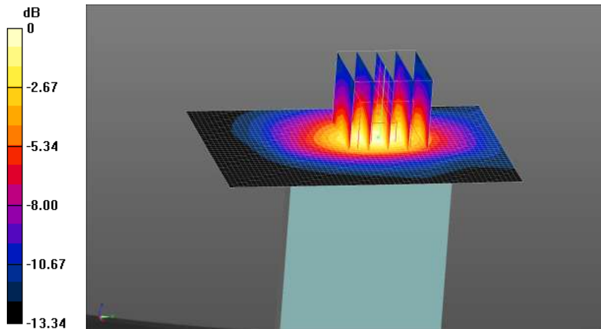
0 dB = 0.136 \text{ W/kg} = -8.66 \text{ dBW/kg}
