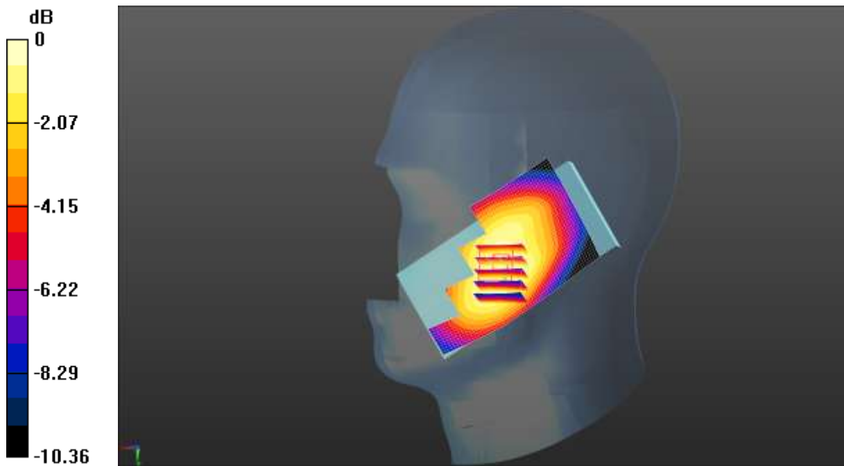
0 dB = 0.415 W/kg = -3.82 dBW/kg
