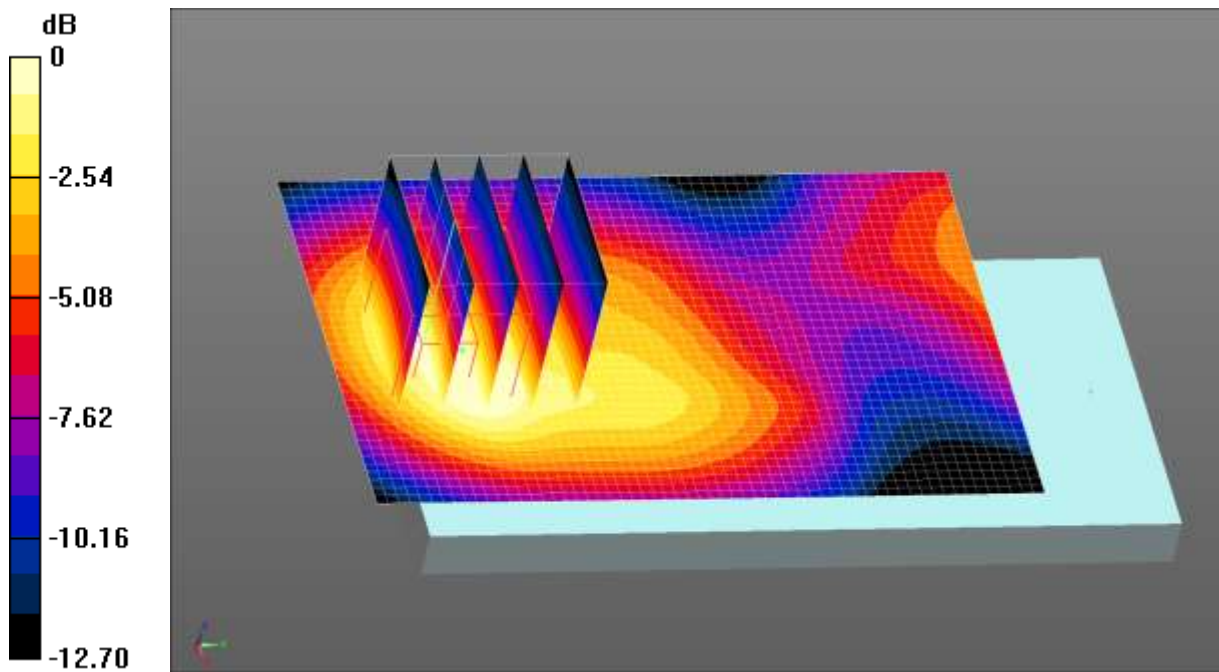
0 dB = 0.271 W/kg = -5.67 dBW/kg
