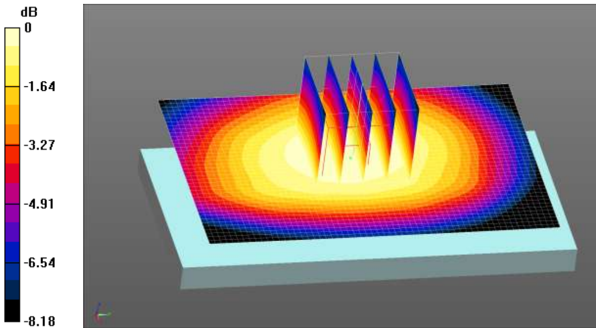
0 dB = 0.537 W/kg = -2.70 dBW/kg
