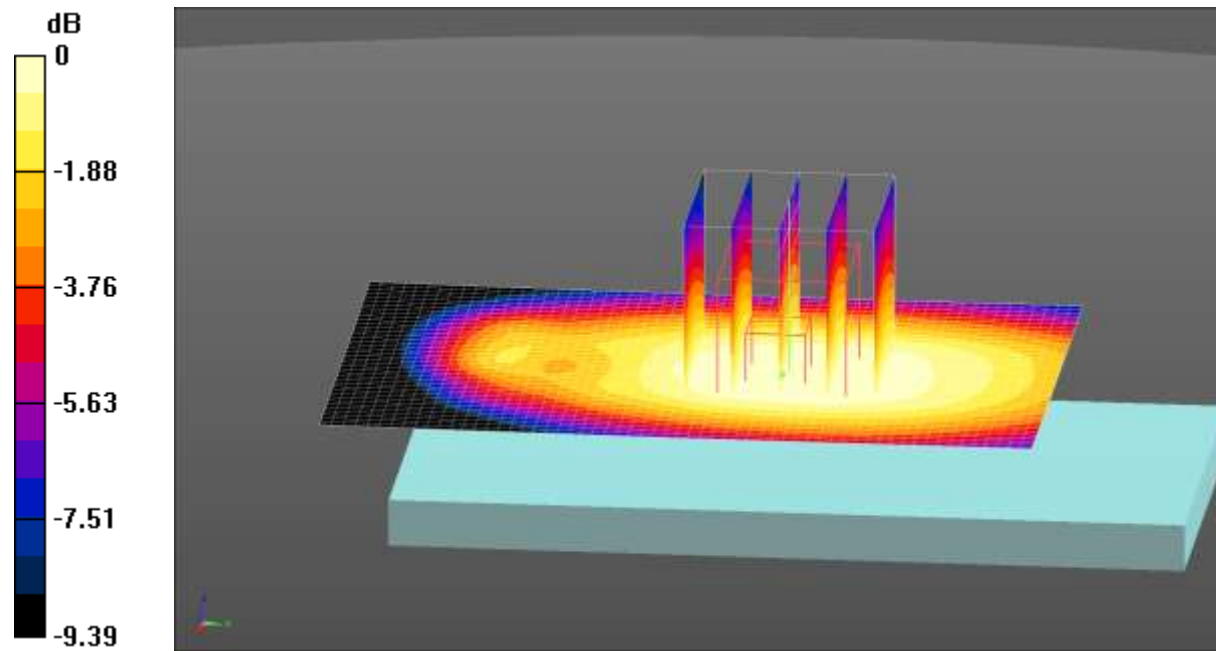
0 dB = 0.736 W/kg = -1.33 dBW/kg
