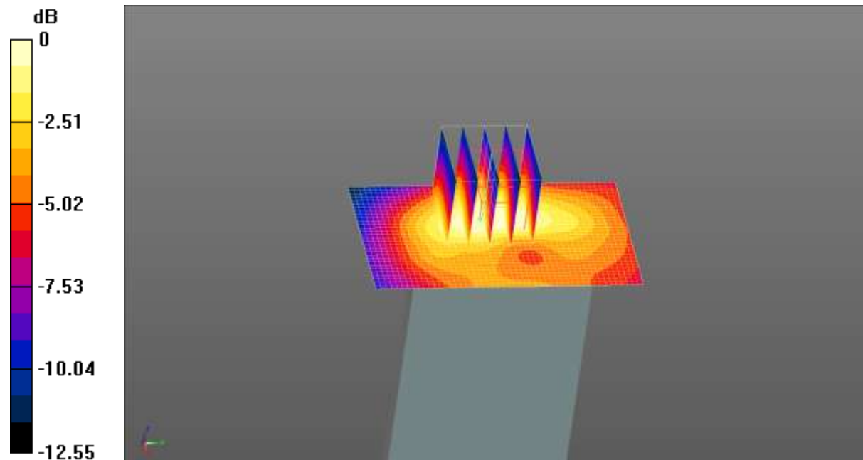
0 dB = 0.162 W/kg = -7.90 dBW/kg
