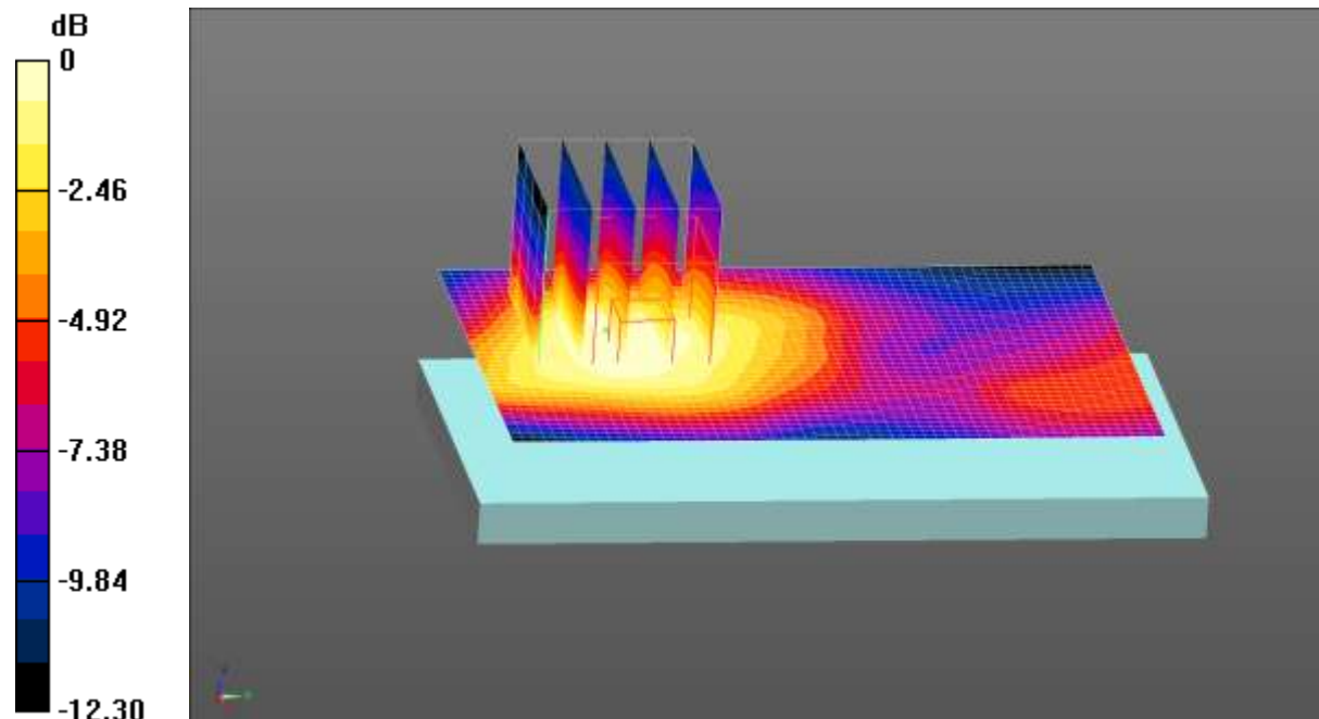
0 dB = 0.0899 W/kg = -10.46 dBW/kg
