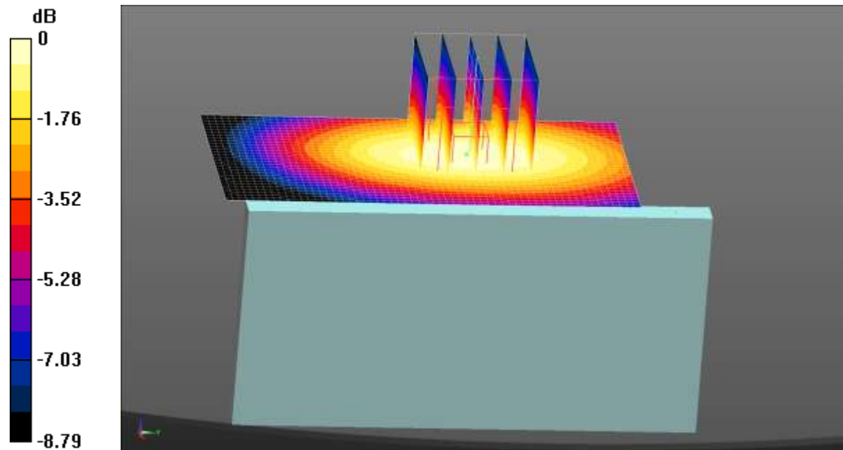
0 dB = 0.242 W/kg = -6.16 dBW/kg
