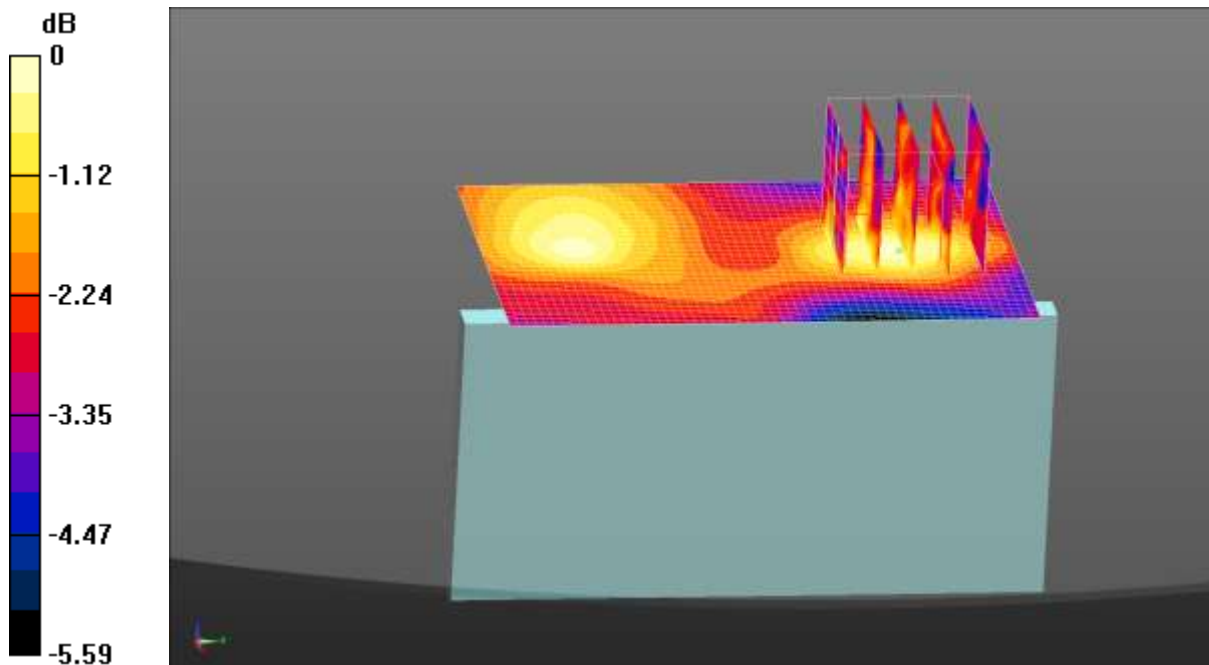
0 dB = 0.0147 W/kg = -18.33 dBW/kg
