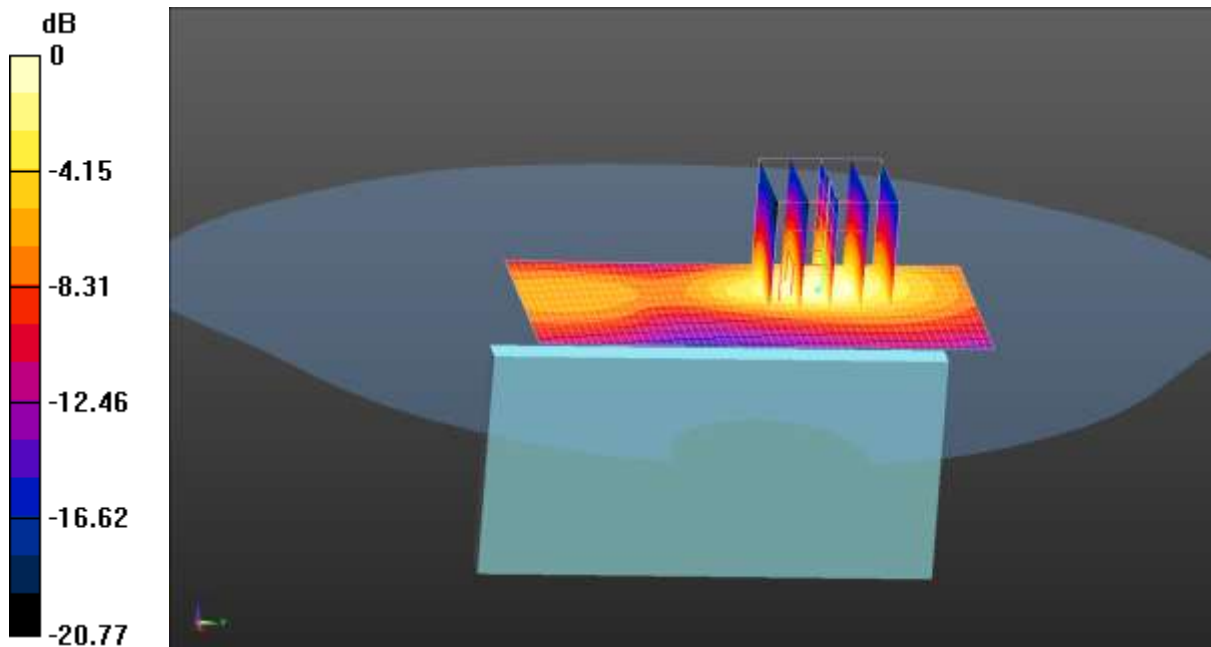
0 dB = 0.165 W/kg = -7.83 dBW/kg
