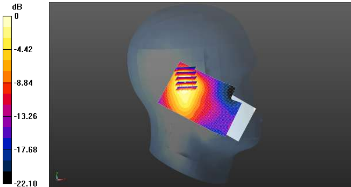
0 dB = 0.190 W/kg = -7.21 dBW/kg
