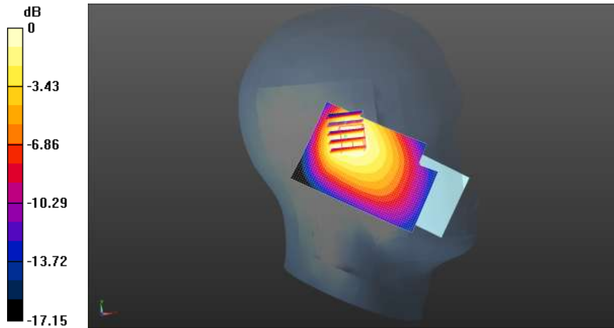
0 dB = 0.605 W/kg = -2.18 dBW/kg
