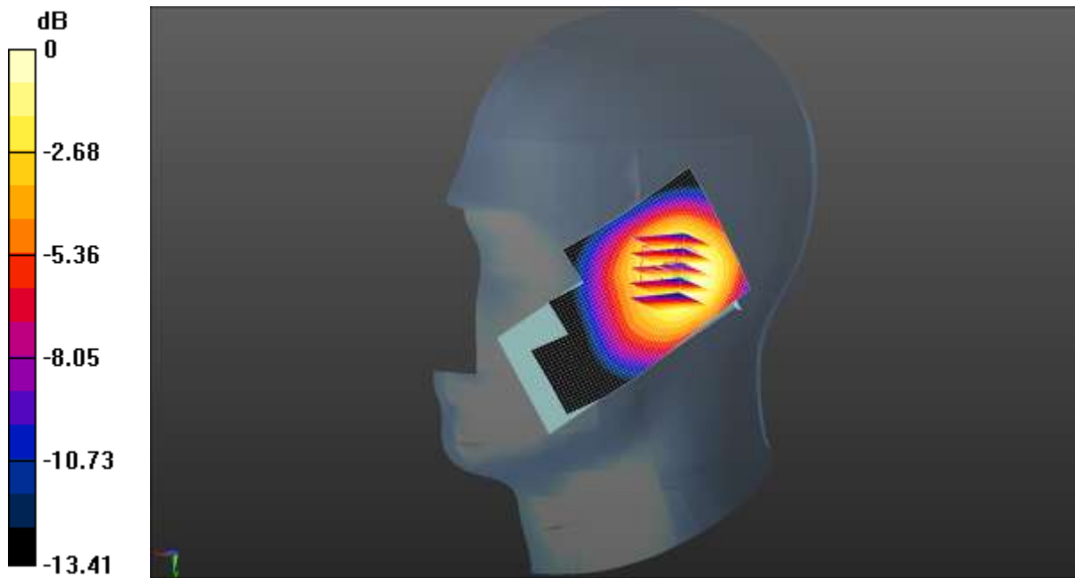
0 dB = 0.705 W/kg = -1.52 dBW/kg
