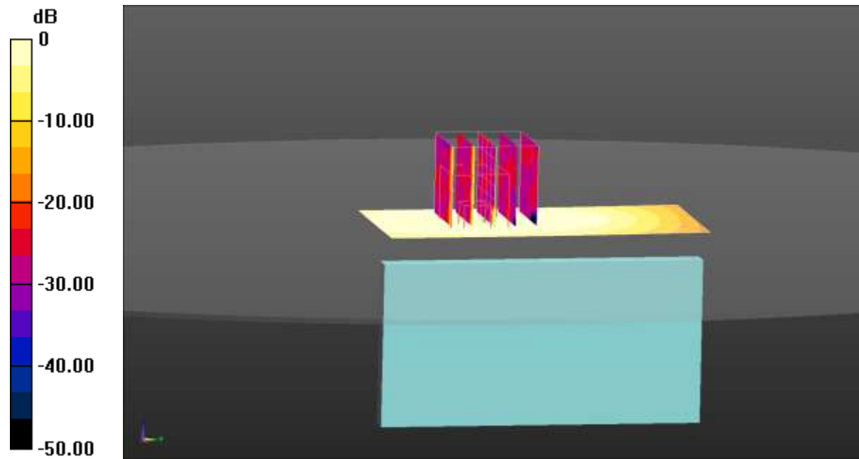
0 dB = 0.167 W/kg = -7.77 dBW/kg
