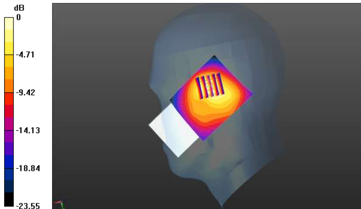
0 dB = 0.899 W/kg = -0.46 dBW/kg
