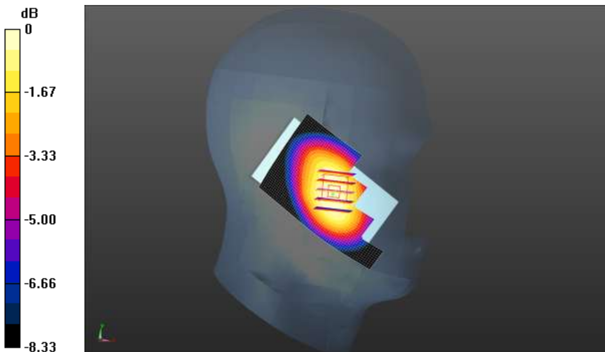
0 dB = 0.783 W/kg = -1.06 dBW/kg
