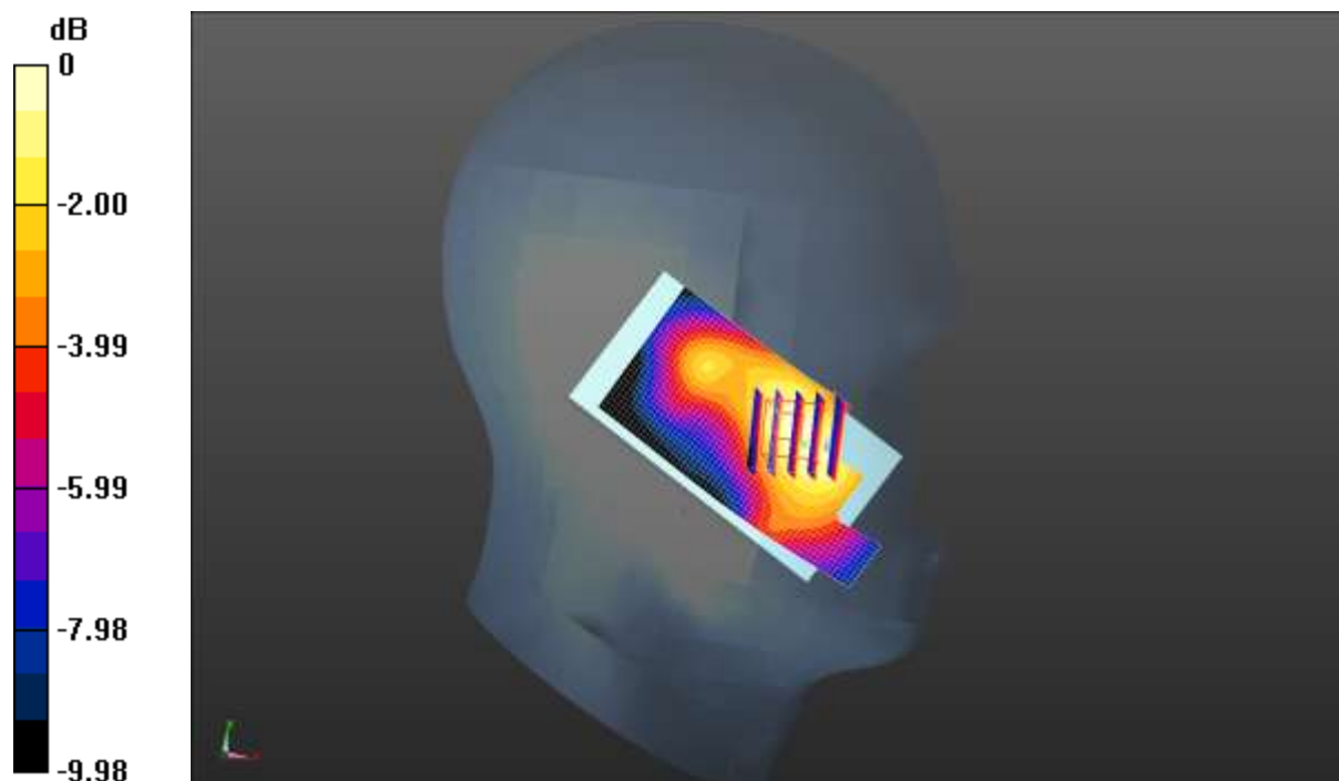
0 dB = 0.0910 W/kg = -10.41 dBW/kg
