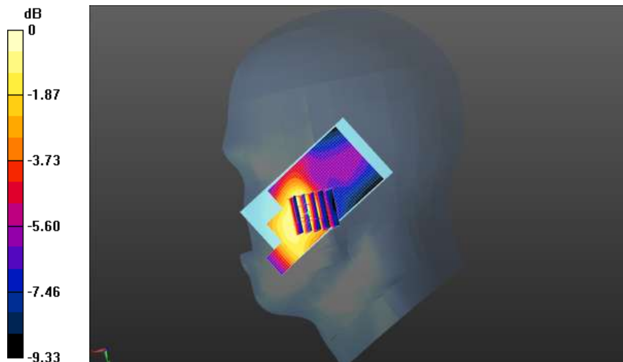
0 dB = 0.0846 W/kg = -10.73 dBW/kg
