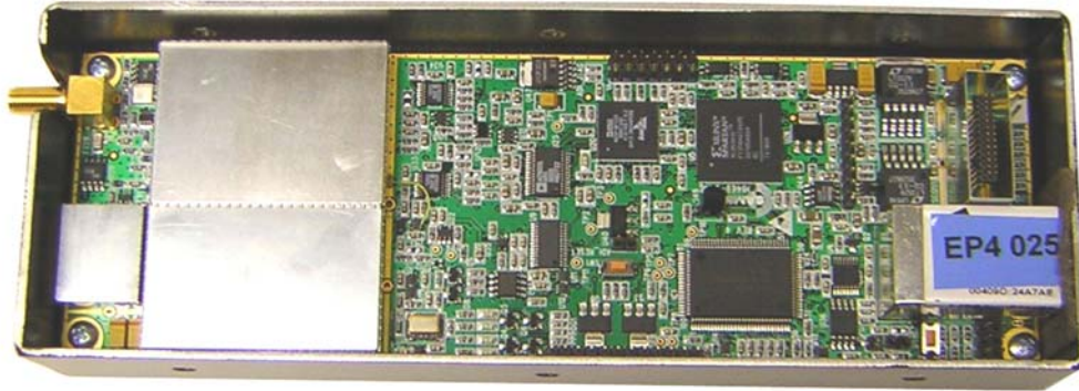
Component Side – Shields Removed
