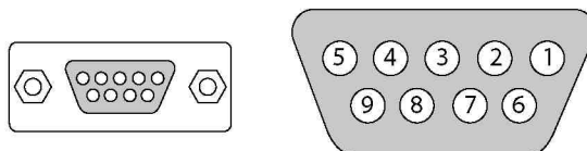
Figure 11: RS-232 Connector
