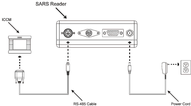
Figure 7: RS-485 Cable Installation
