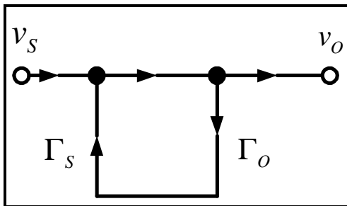
Figure 8.4-1 Signal flow graph of the Tach NXT TX/power meter interface.
