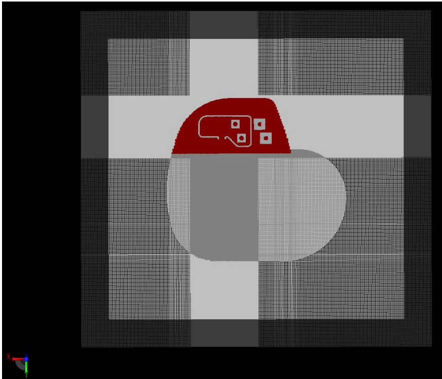
Figure 8.1-2 One layer of the meshed XFDTD volume space.
