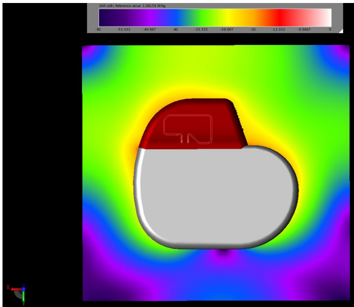
Figure 8.3-3 SAR distribution in tissue surrounding the implant.
