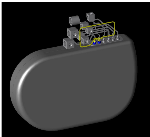
Figure 7.1-3 Antenna structure #1.
