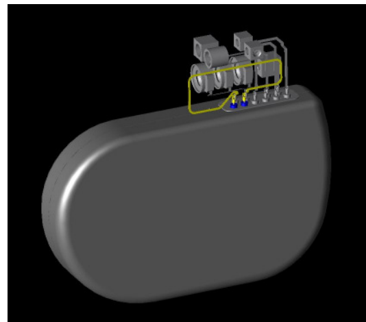
Figure 7.1-4 Antenna structure #2.
