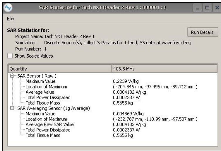
Figure 8.3-2 Summary of SAR statistics for antenna structure #2.
