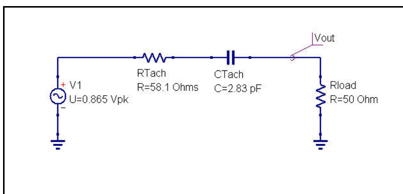
Figure 8.4-2 Determination of equivalent source voltage
