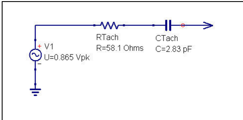
Figure 8.2-1 Thevenin equivalent circuit of Tach NXT RF transmitter.
