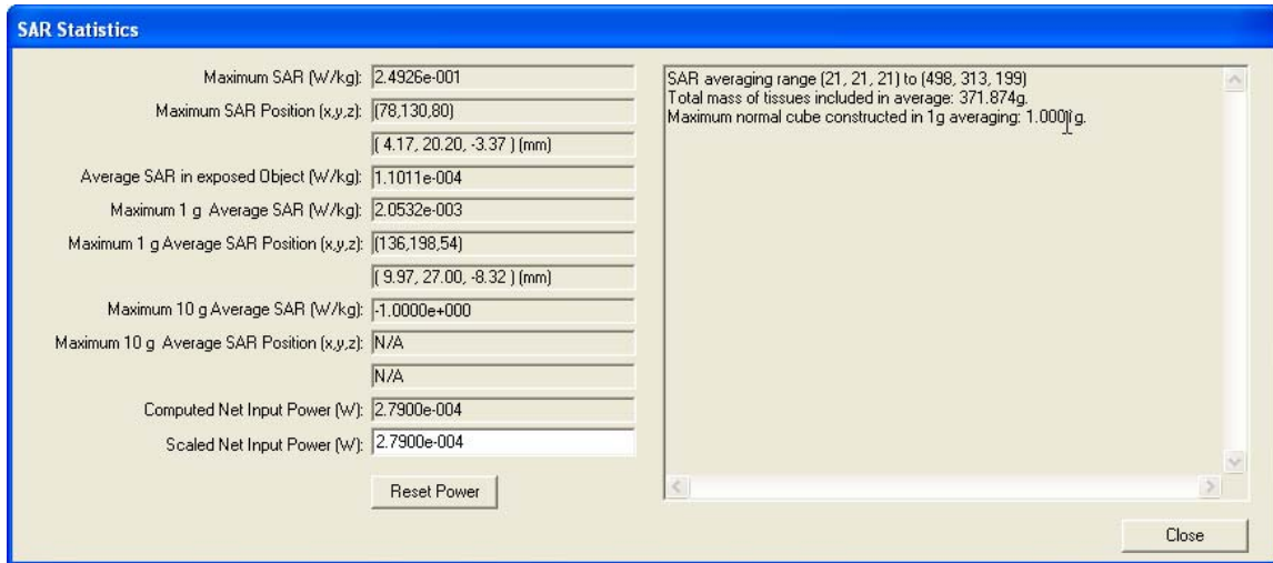
Figure 8.2.1 FDTD Summary of SAR Statistics
