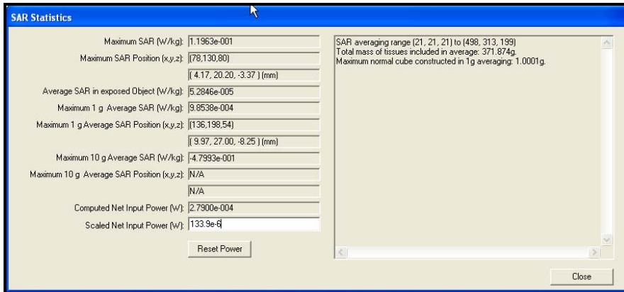
Figure 8.2.1 FDTD Summary of SAR Statistics
