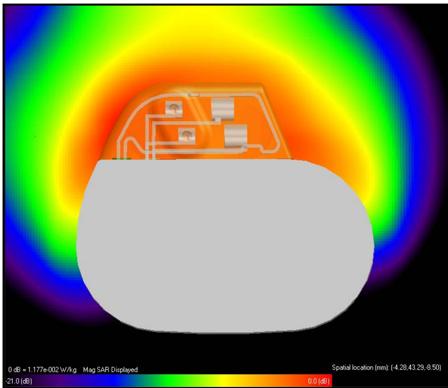
Figure 8.2.2 Intensity of the SAR distribution around the implant.
