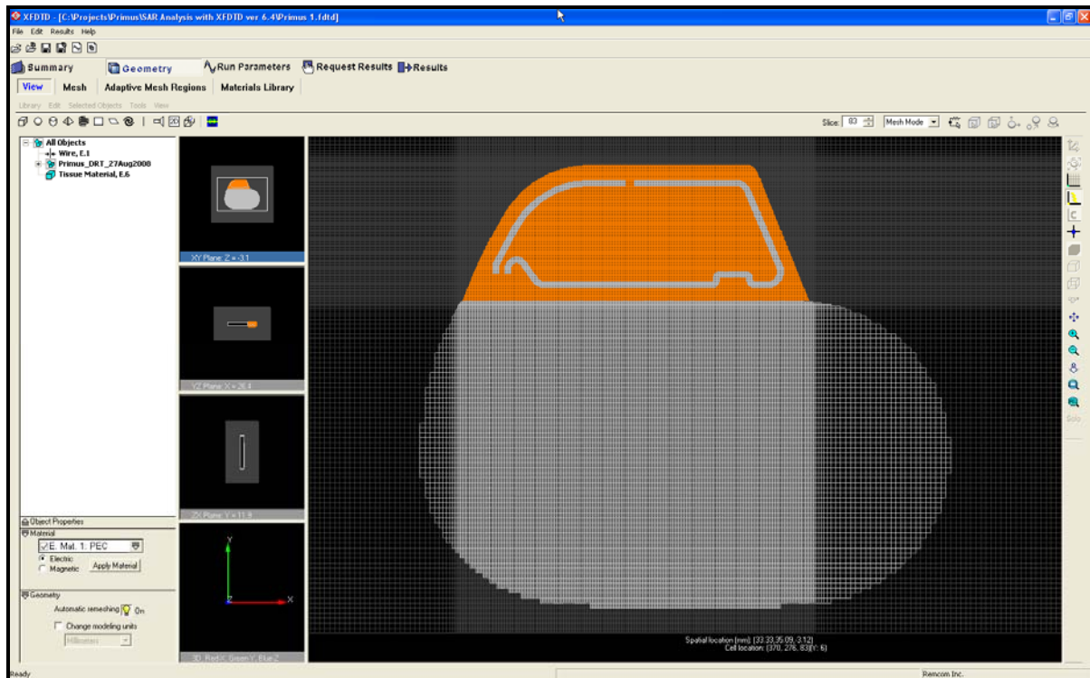
Figure 8.1.2 Meshed XFDTD problem space showing the pacemaker’s case, epoxy header, and antenna structure.
