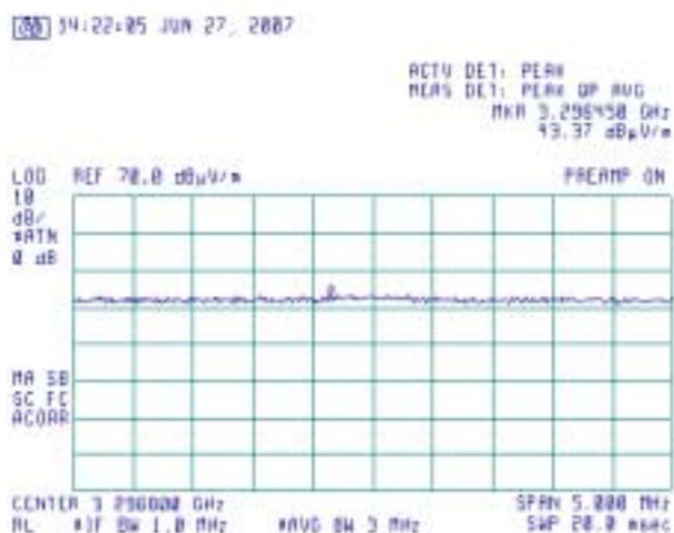
Plot 7.4.23 Radiated emission measurements at the 4 th harmonic
