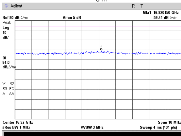
Plot 8.4.42 Radiated emission measurements at the 9 th harmonic
