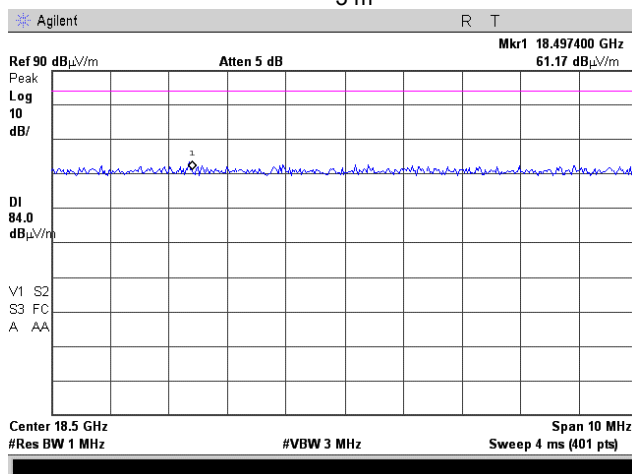
Plot 8.4.44 Radiated emission measurements at the 10 th harmonic
