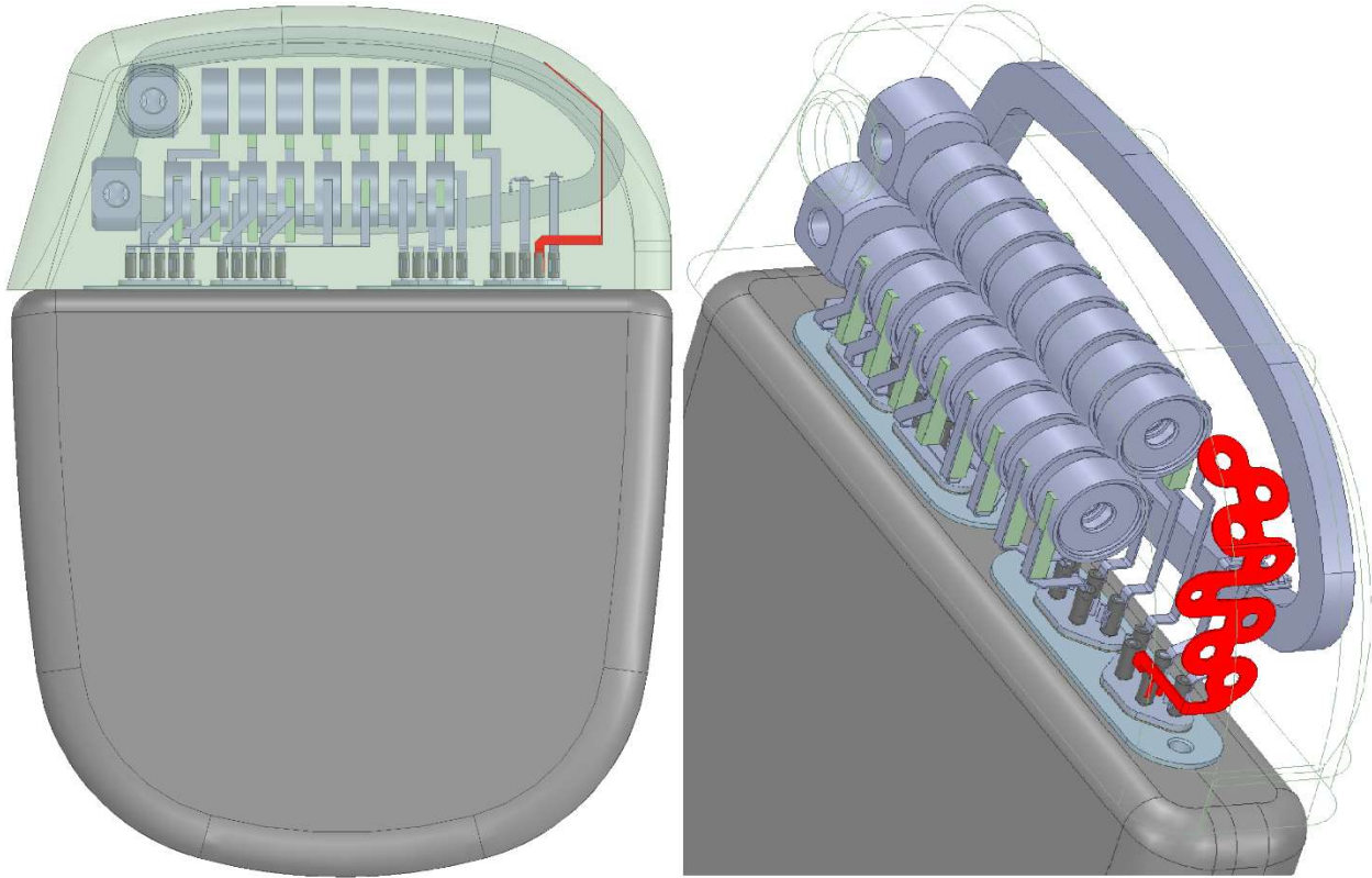
Figure 1 BLE antenna in device header
