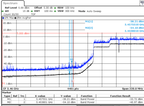
BE - R Low Freq Section, Peak, RMS – CH114
