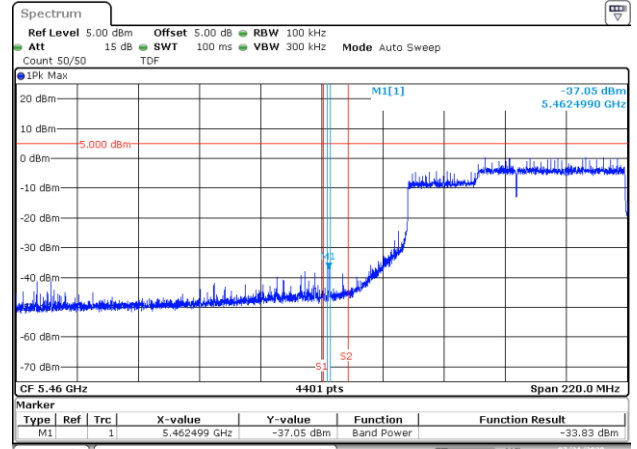
BE - NR Low Freq Section, Peak – CH114
