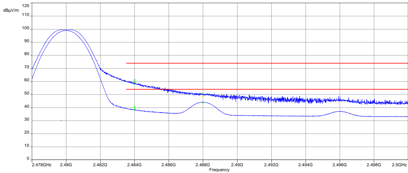
Plot 2: Upper restricted band, 1 Msps, on-board antenna
