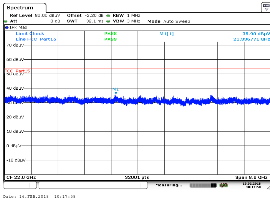
Plot 4: 18 GHz to 26 GHz, RX / idle – mode, vertical &amp; horizontal polarization, external antenna
