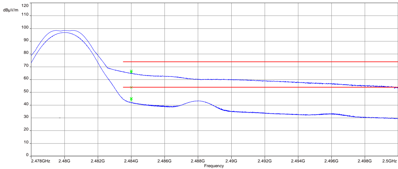
Plot 8: Upper restricted band, 2 Msps, external antenna
