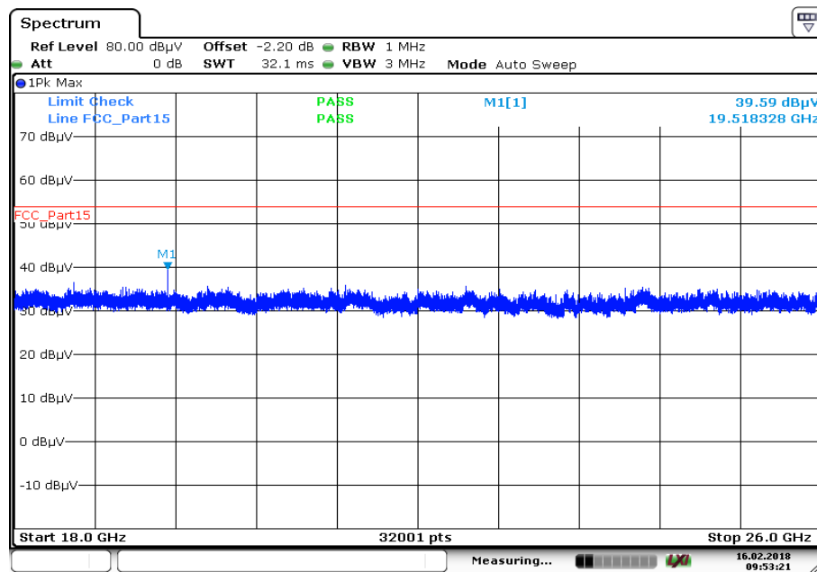
Plot 4: 18 GHz to 26 GHz, TX mode, 2440 MHz, vertical &amp; horizontal polarization, 1 Msps, on-board antenna
