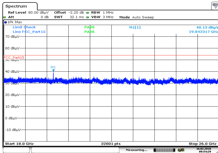
Plot 6: 18 GHz to 26 GHz, TX mode, 2480 MHz, vertical &amp; horizontal polarization, 1 Msps, on-board antenna
