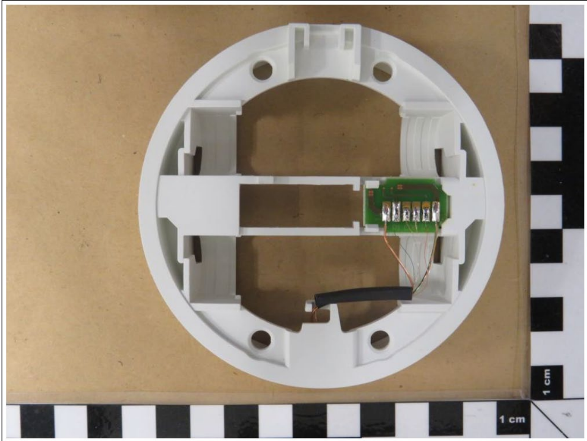
PGH INNER BRACKET TOP SIDE
