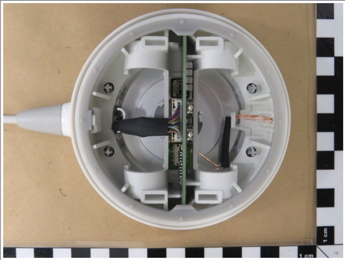
PGH TOP SIDE
