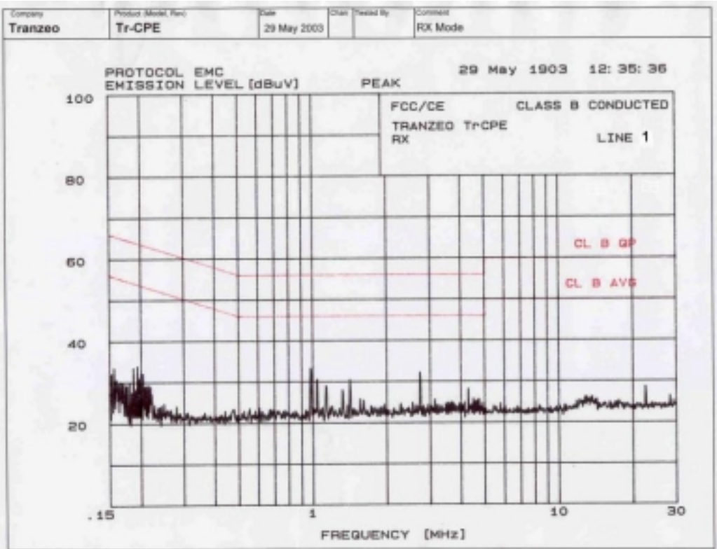
Line 1 Conducted Emissions
