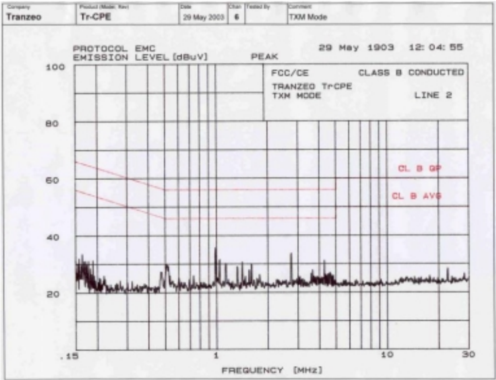
Line 2 Conducted Emissions
