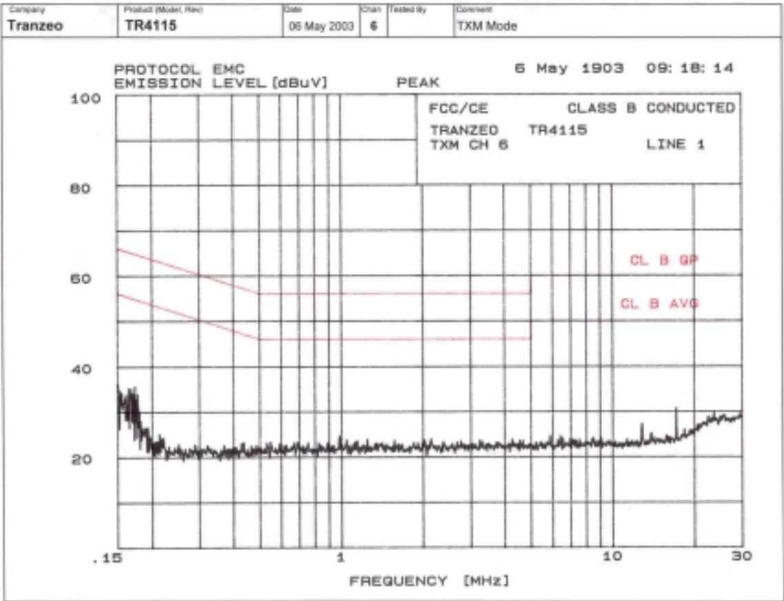
Line 1 Conducted Emissions
