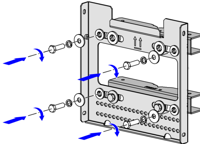
Figure 2-15 Fix Wall-mounting Components and Pole Clips
