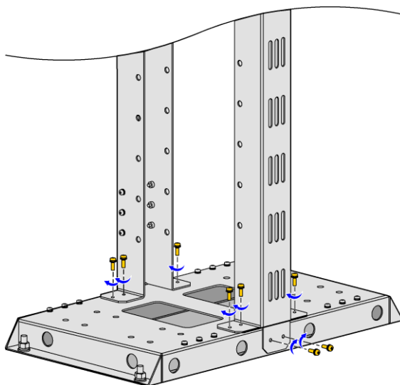
Figure 2-26 Install the Vertical Shaft and the Bottom Plate
