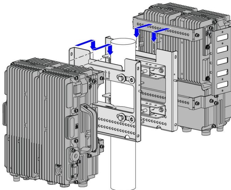
Figure 2-17 Hang the Devices on the Wall-mounting Components
