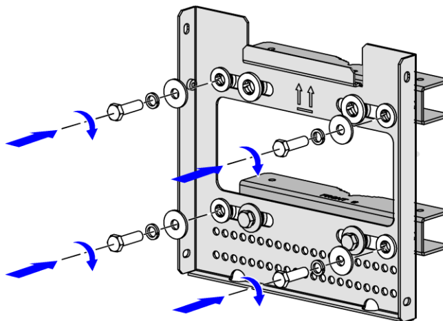
Figure 2-8 Fix Wall-mounting Components and Pole Clips
