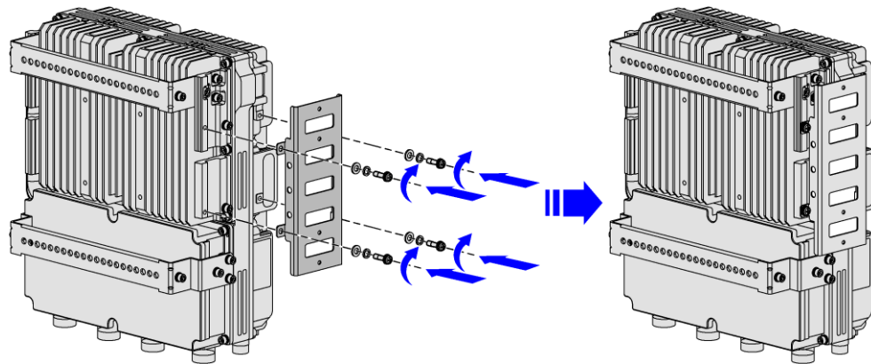
Figure 2-7 Attach Installation Accessory for Lightning Protection Box
