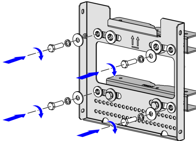
Figure 2-21 Fix Wall-mounting Components and Pole Clips
