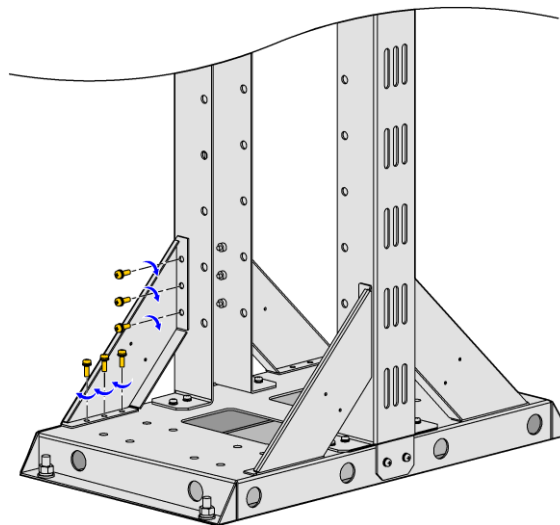
Figure 2-28 Install the Slanted Rack
