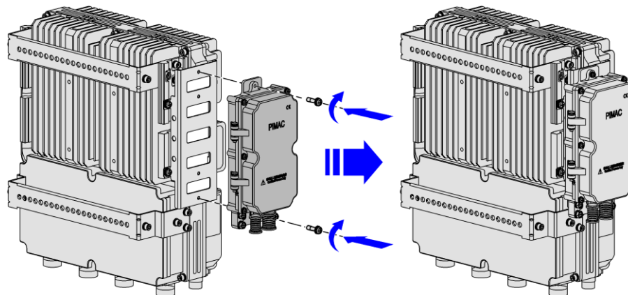
Figure 2-19 Attach Lightning Protection Box
