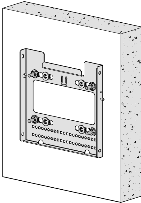
Figure 2-3 Wall-mounting Components Fixed on Wall
