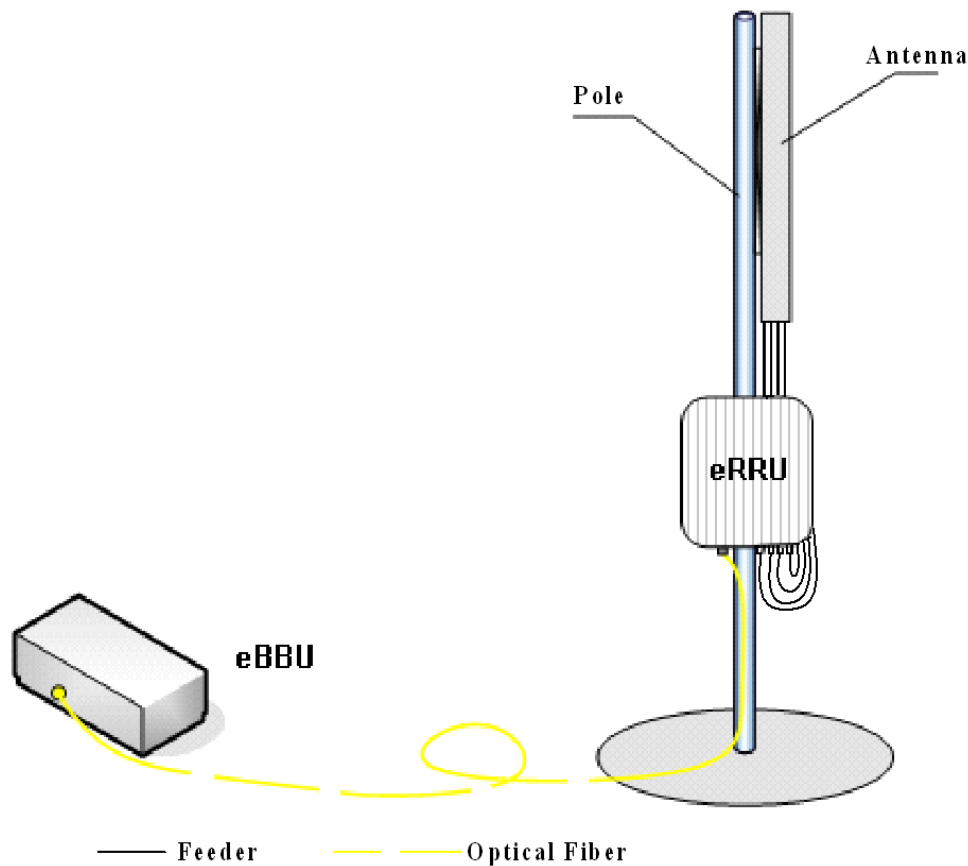
Figure 1-1 LEMKO Distributed eNodeB Solution
