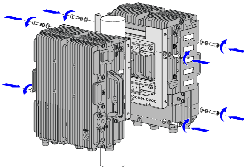
Figure 2-18 Fix the Devices on the Wall-mounting Components
