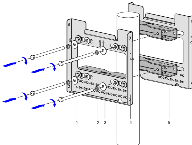
Figure 2-16 Fix Wall-mounting Components and Pole Clips on Pole
