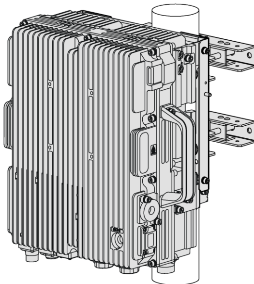
Figure 2-12 LMKT RL1F22 Is Installed on Pole
