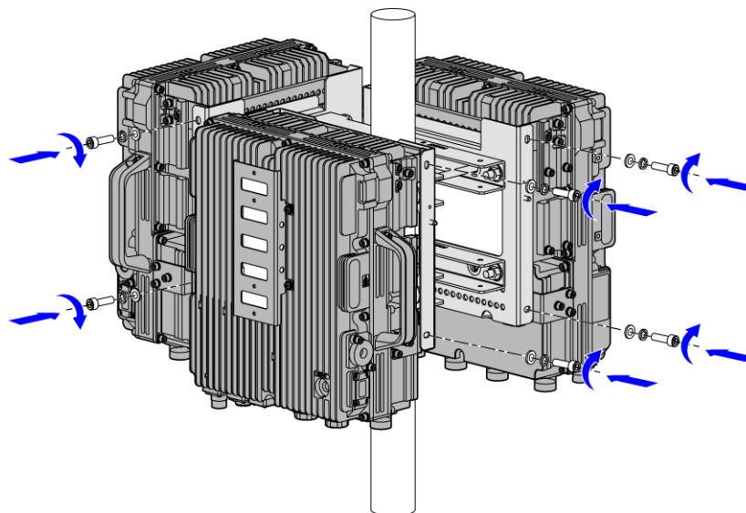
Figure 2-24 Hang the Devices on the Wall-mounting Components
