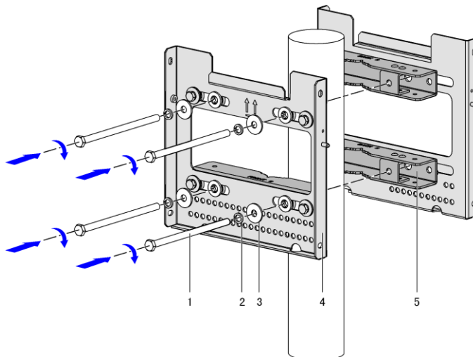
Figure 2-22 Fix Wall-mounting Components and Pole Clips on Pole
