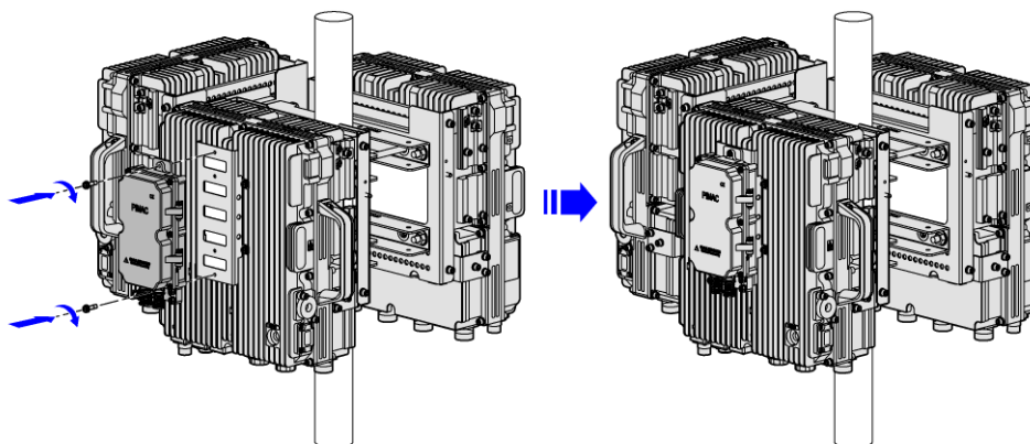
Figure 2-25 Attach Lightning Protection Box
