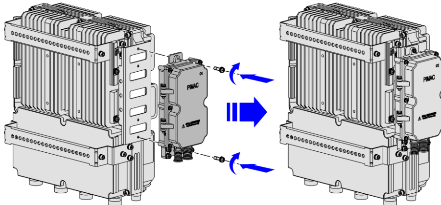
Figure 2-13 Attach Lightning Protection Box
