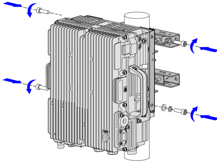
Figure 2-11 Fix the Device on the Wall-mounting Components
