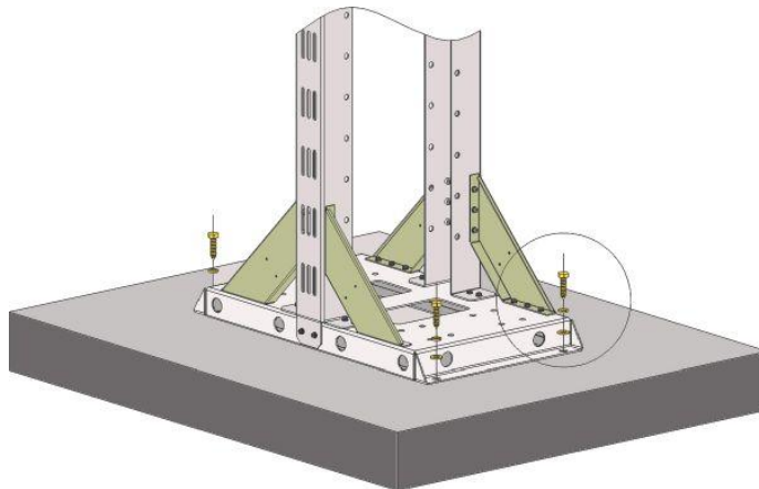
Figure 2-32 Install the Gantry on Wooden Floor
