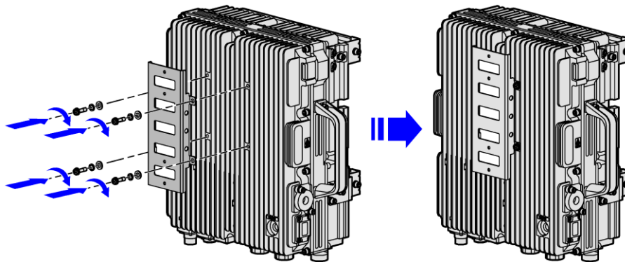
Figure 2-20 Attach Installation Accessory for Lightning Protection Box
