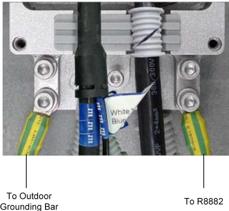
Figure 2-41 PIMDC Grounding Bar Connection
