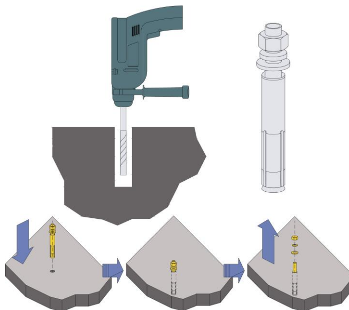
Figure 2-30 Install the Expansion Bolt
