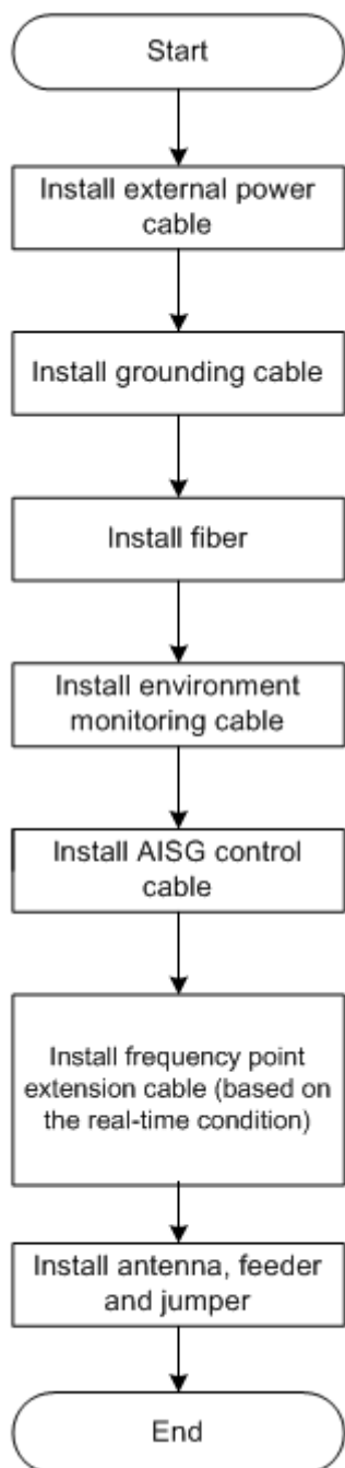
Figure 2-34 External Cable Installation Flow
