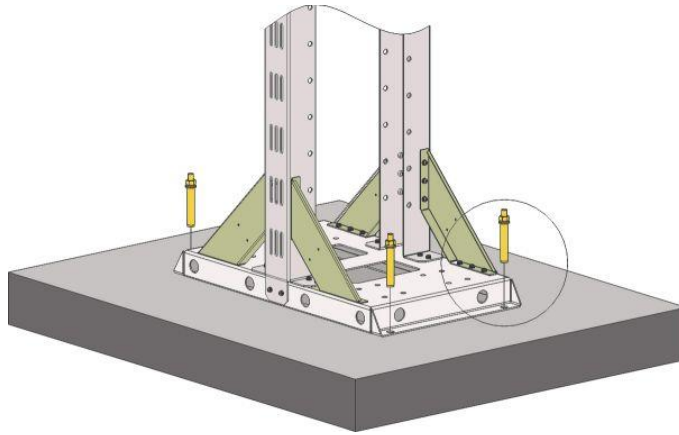
Figure 2-31 Install the Gantry on Concrete Floor
