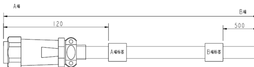
Figure 2-47 Environment Monitor Cable
