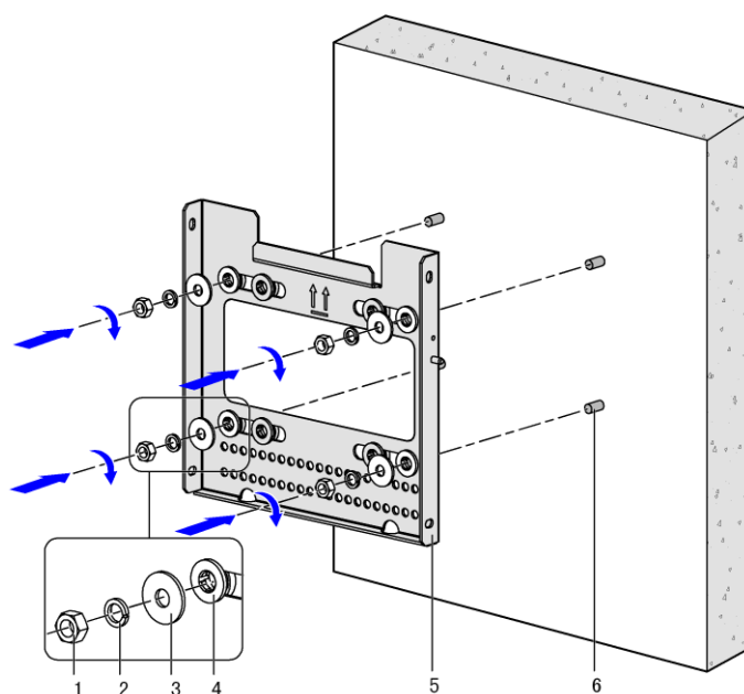
Figure 2-2 Installing Wall-mounting Components
