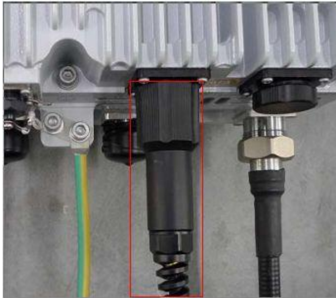
Figure 2-46 Tighten Connection
