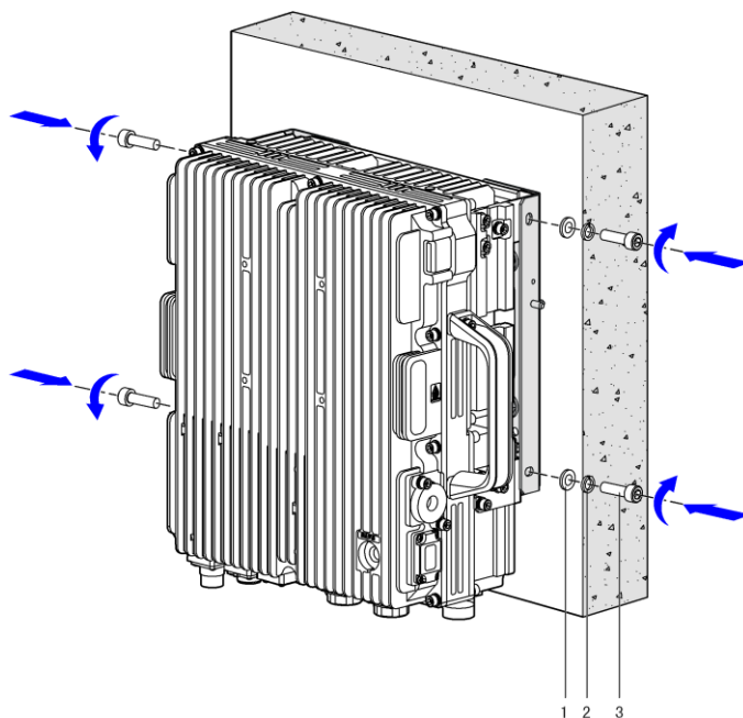
Figure 2-5 Fasten Device
