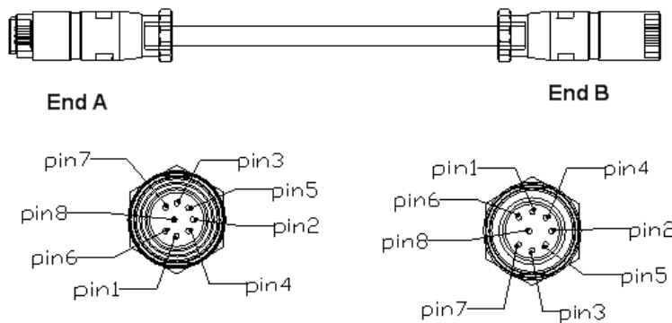
Figure 2-49 Structure of AISG Control Cable
