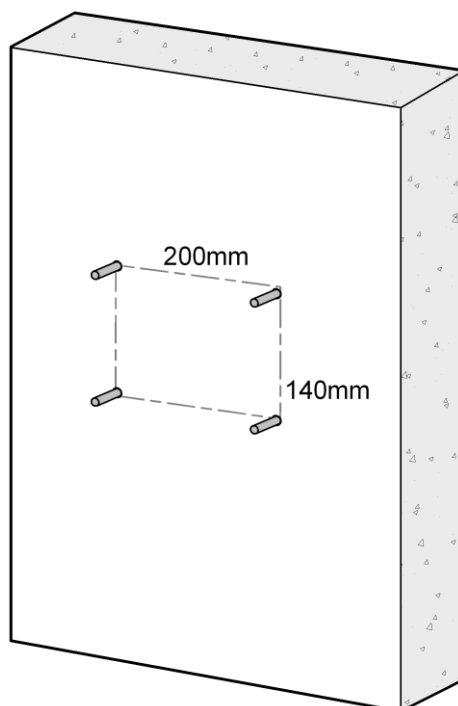
Figure 2-1 Template Hole Position
