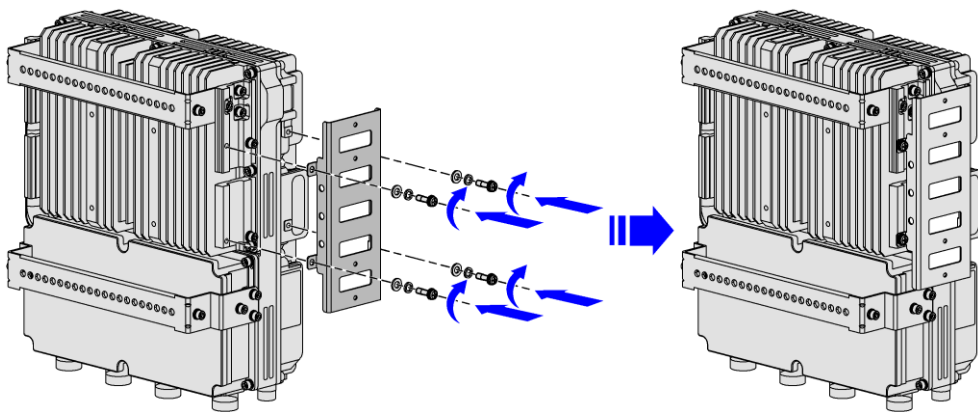
Figure 2-14 Attach Installation Accessory for Lightning Protection Box
