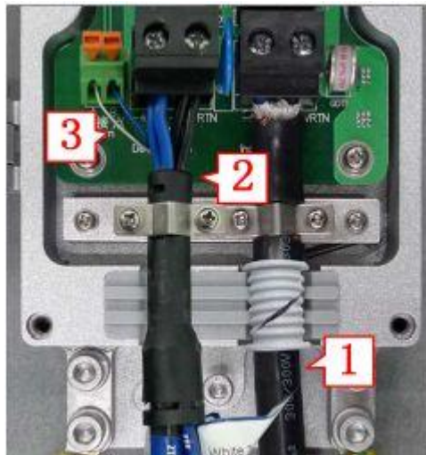
Figure 2-35 PIMDC Power Cable Connection
