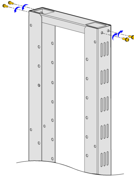
Figure 2-27 Fasten the Vertical Shaft and the Cover Plate
