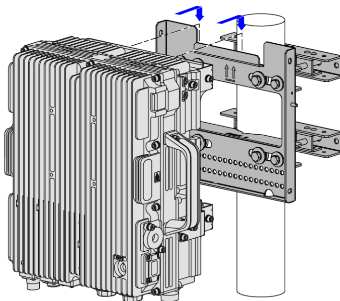
Figure 2-10 Hang the Device on the Wall-mounting Components
