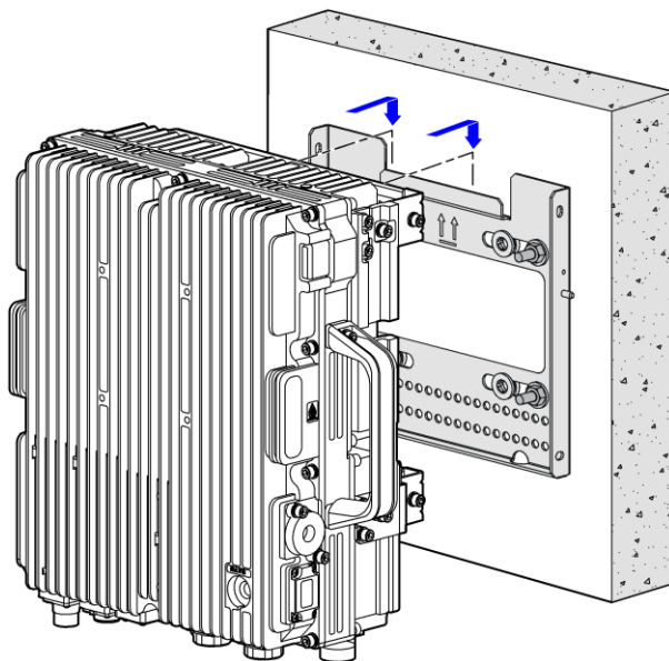
Figure 2-4 Hang the Device on the Wall-mounting Components
