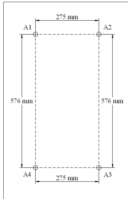
Figure 2-29 Mark the Drilling Holes Position
