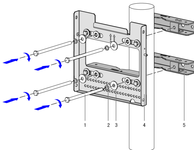
Figure 2-9 Fix Wall-mounting Components and Pole Clips on Pole
