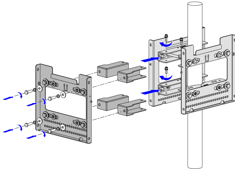
Figure 2-23 Fix the Third Wall-mounting Components
