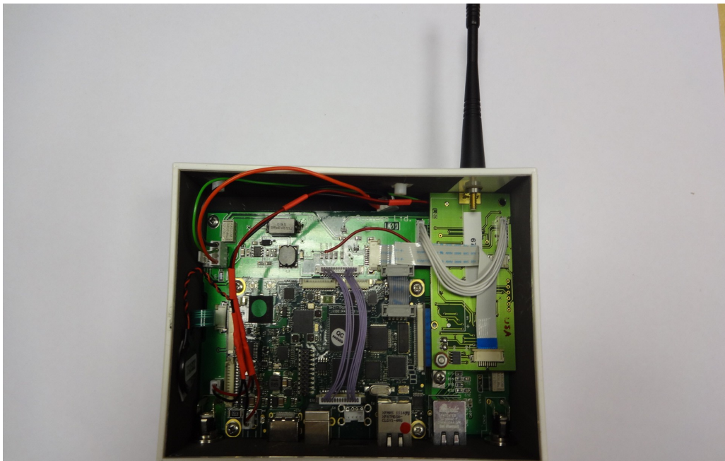
Internal view
