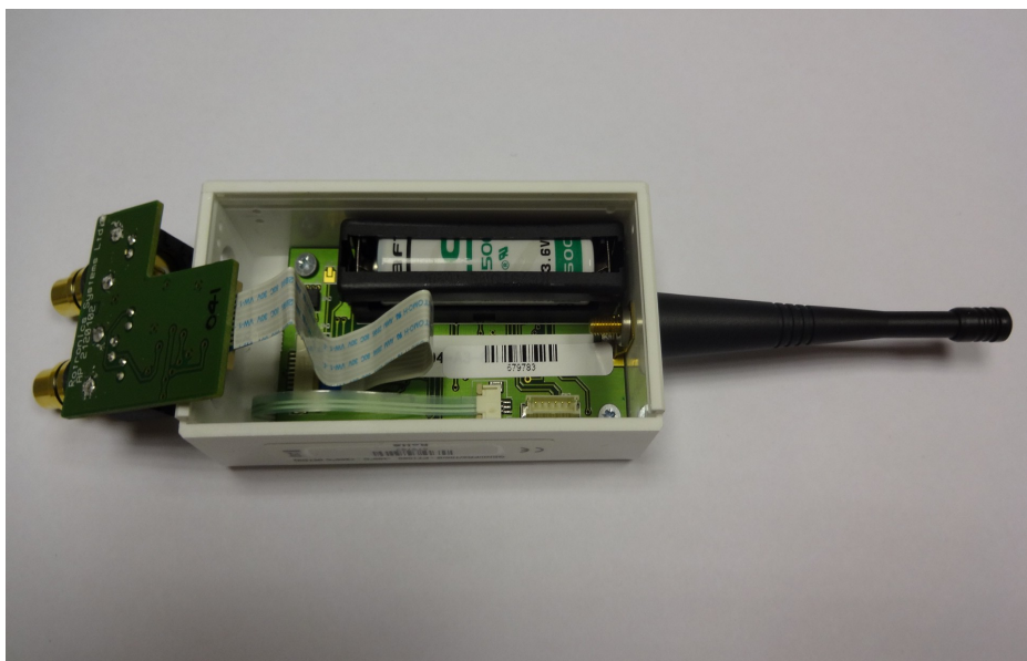
Temperature sensor board removed – switch selectable options A & B
