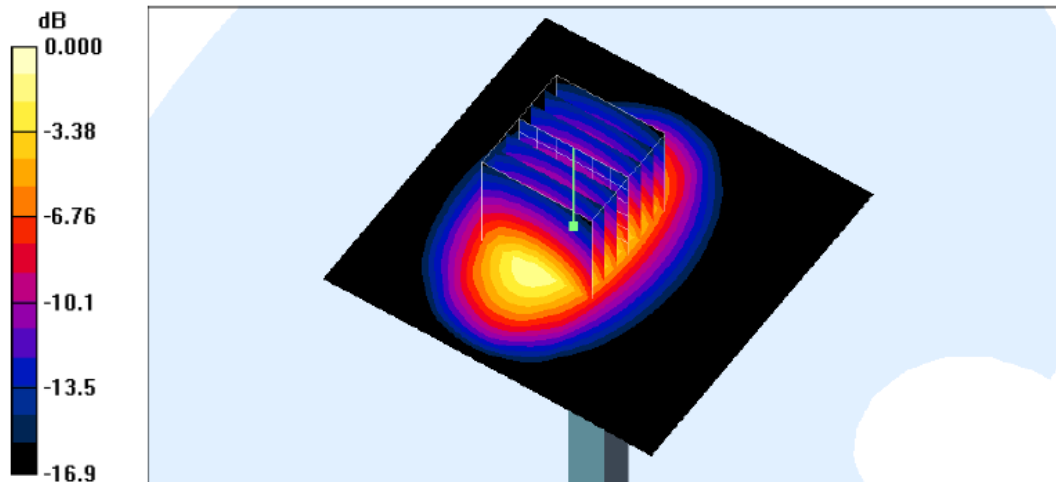
0 dB = 4.60mW/g
