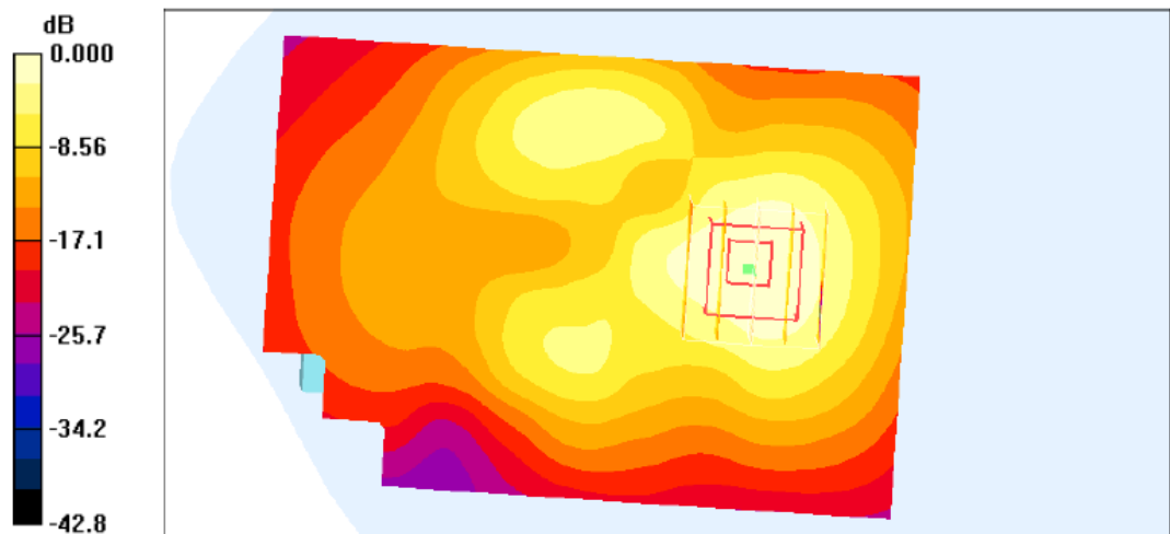
0 dB = 1.15mW/g
