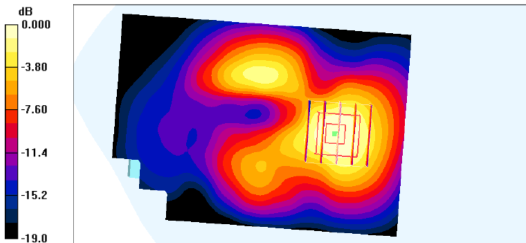
0 dB = 1.06mW/g
