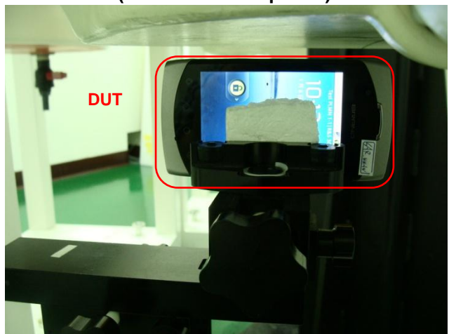
Left of the DUT with Phantom 1 cm Gap (DUT without Earphone)
