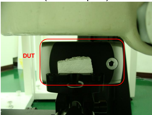
Right of the DUT with Phantom 1 cm Gap (DUT without Earphone)
