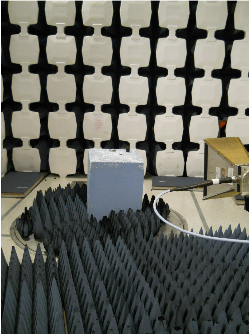
Radiated EMI
