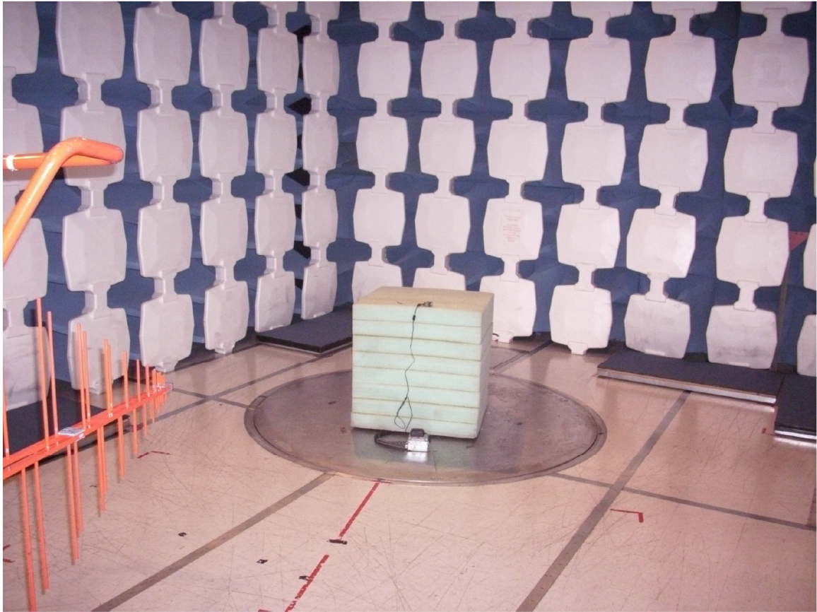
Radiated EMI
