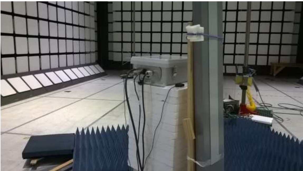
Figure 4 - Radiated Emissions Test Setup, 1GHz - 25GHz, Panel Antenna
