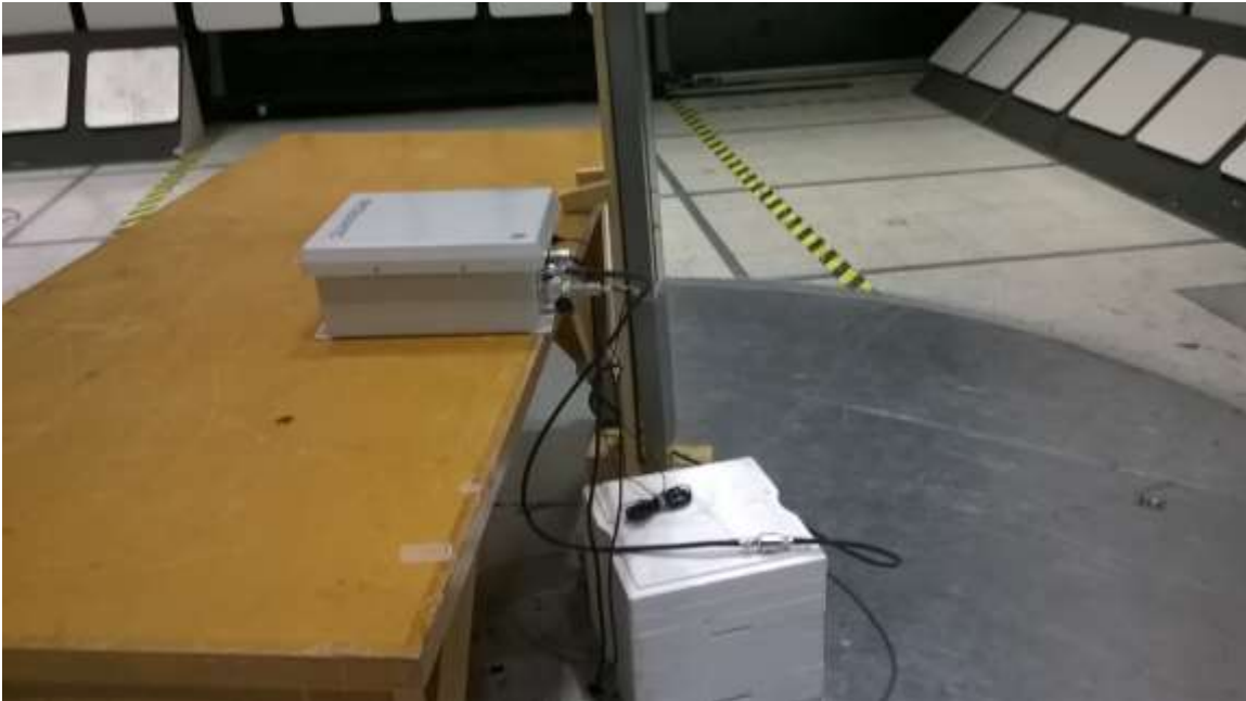
Figure 3 - Radiated Emissions Test Setup, 30MHz – 1GHz, Panel Antenna
