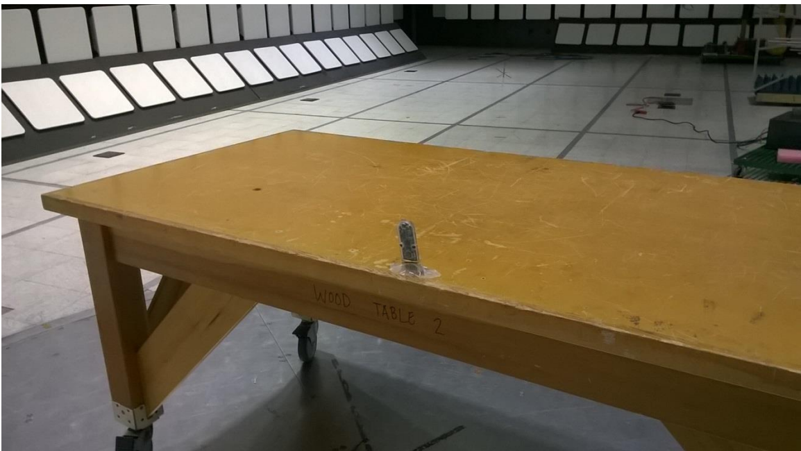
Figure 2 - Radiated Emissions Test Setup, Vertical, 30MHz – 1GHz
