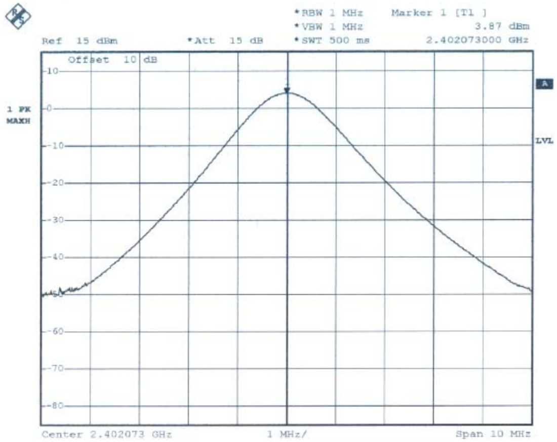
Plot 1 (Channel 00)
