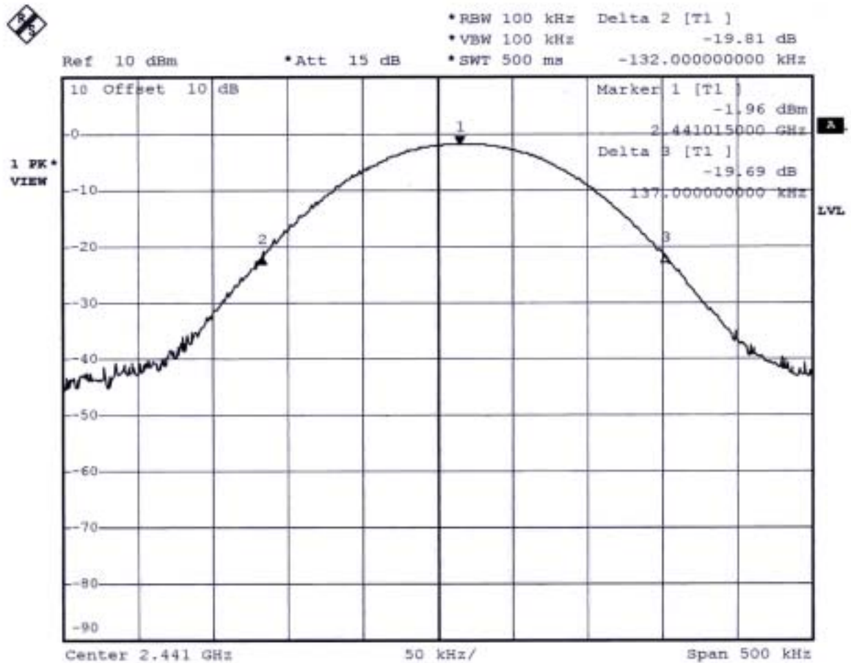
Plot 2 (Channel 39)
