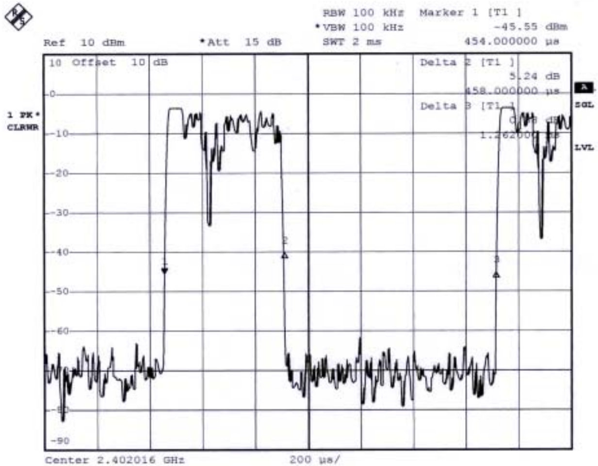
Plot 1 (Channel 00)
