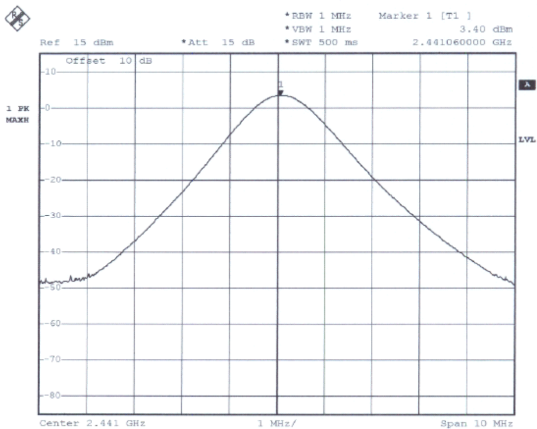
Plot 2 (Channel 39)
