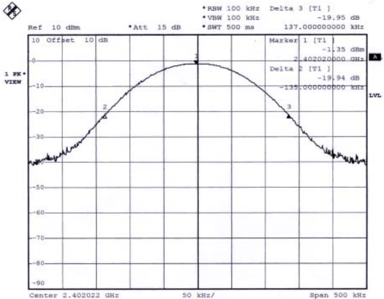
Plot 1 (Channel 00)
