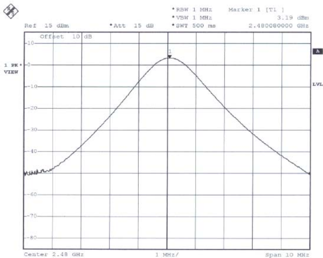
Plot 3 (Channel 78)
