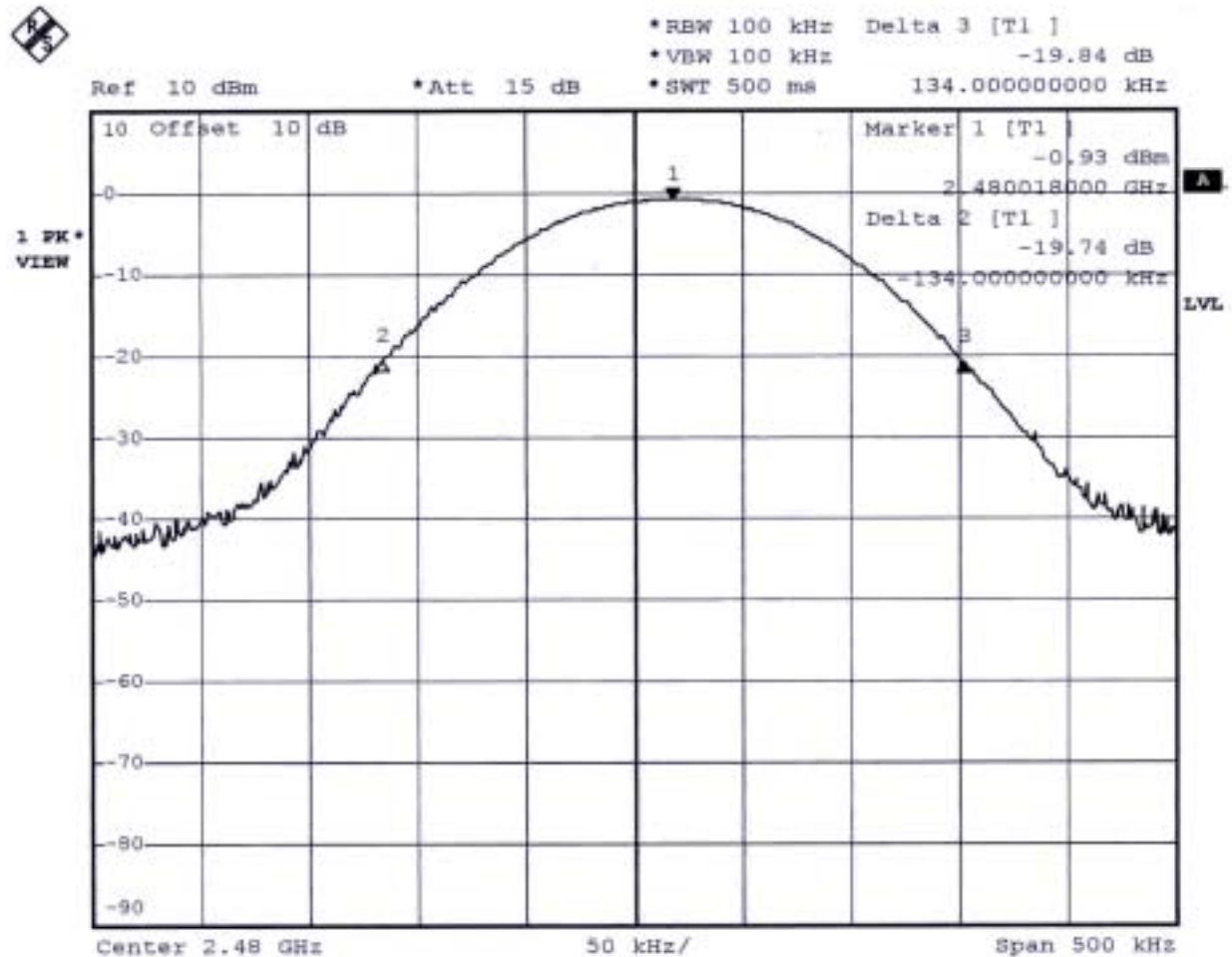
Plot 3 (Channel 78)
