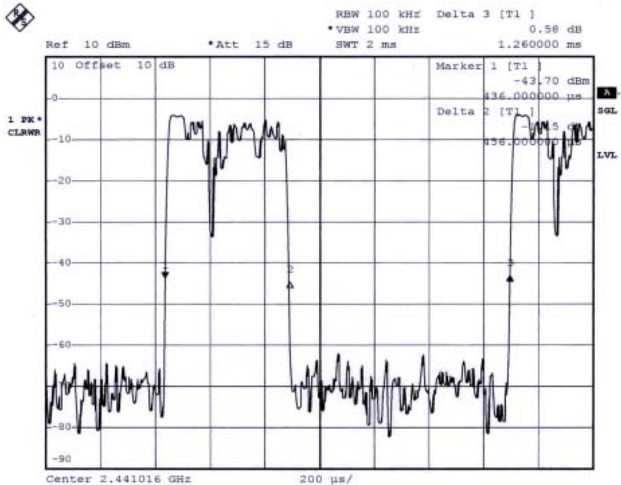
Plot 2 (Channel 39)
