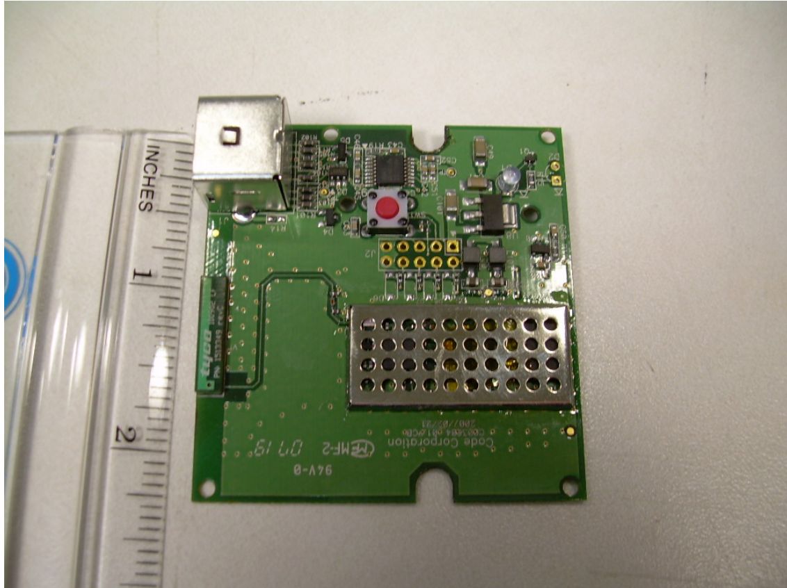
Top Side of PCB
