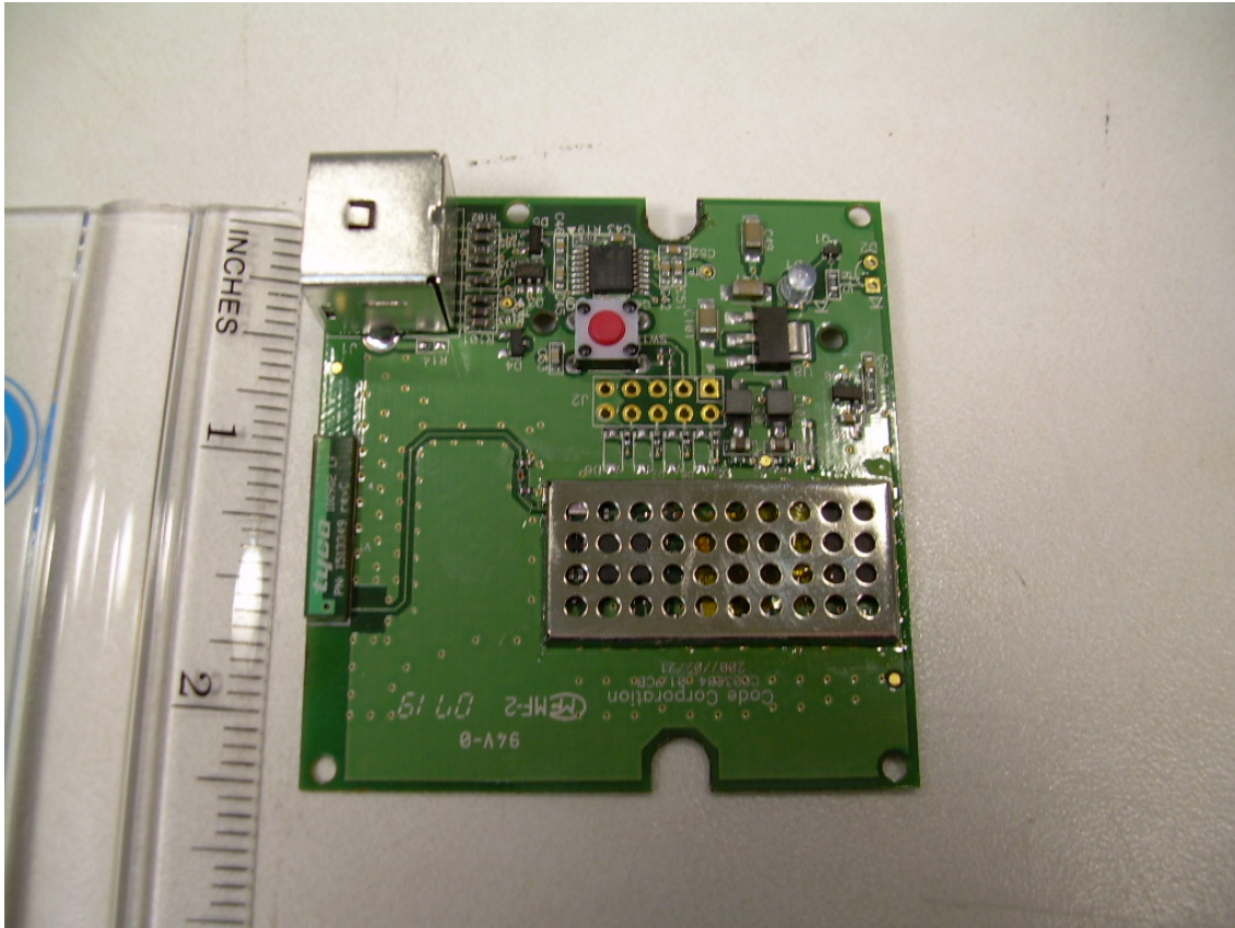
Photograph 5 - Top Side of PCB
