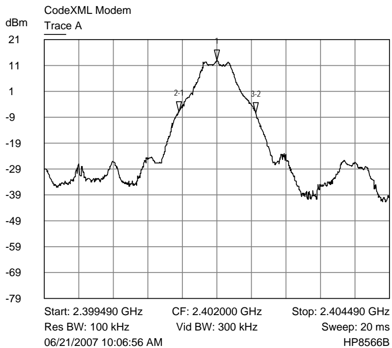
Trace A lower channel output band width plot
