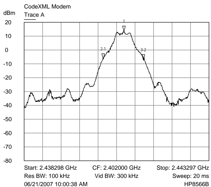
Trace A middle channel output band width plot
