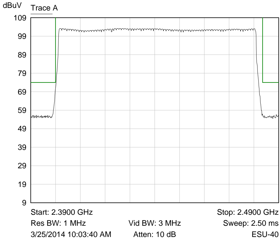
Plot of the Emission in the 2400 – 2483.5 MHz Band While Hopping
