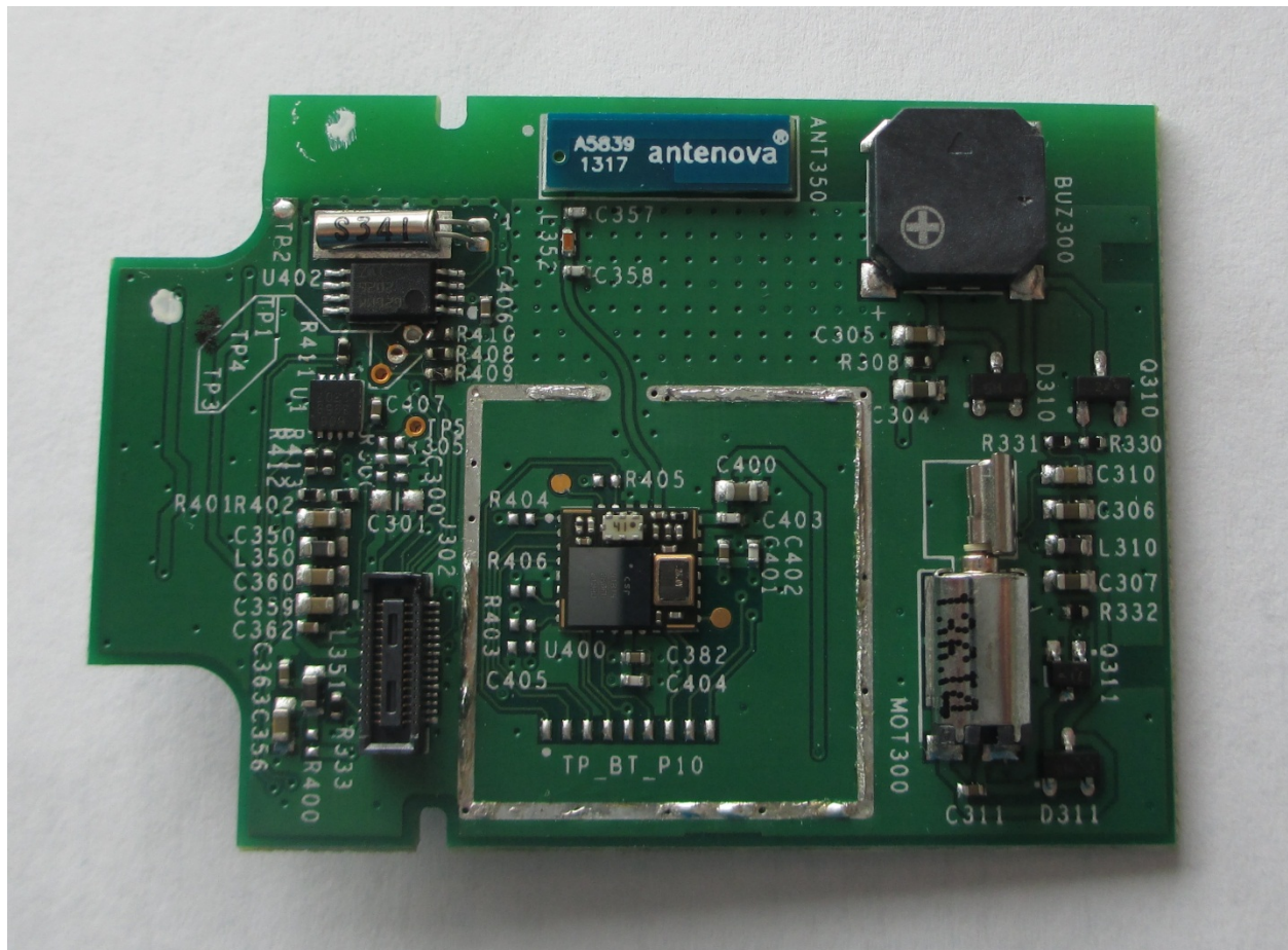
View of the Circuitry Under the RF Shield – Configuration with RTC and Apple Chip
