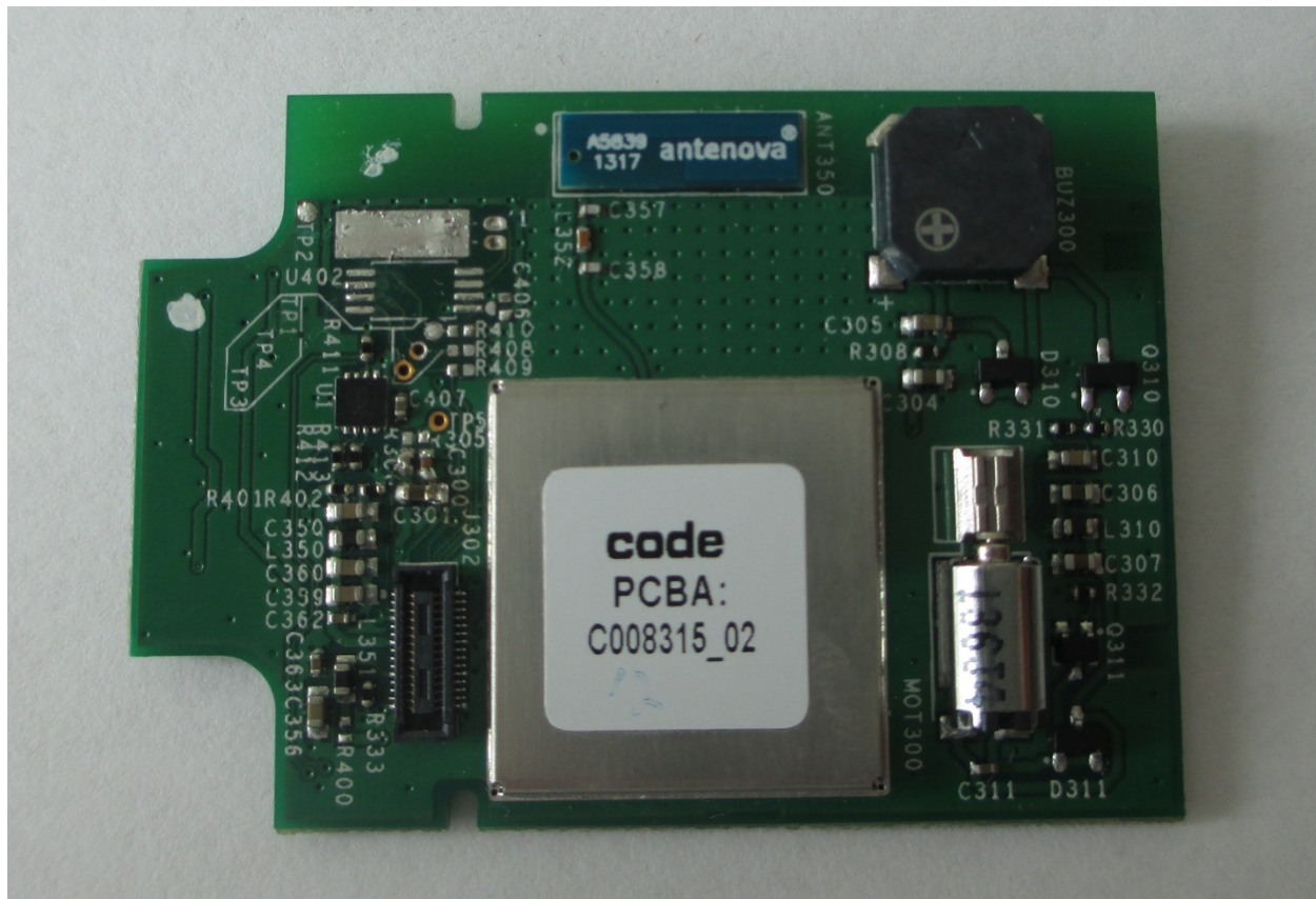
View of the Bottom of the PCB – Configuration With Apple IC, Without RTC
