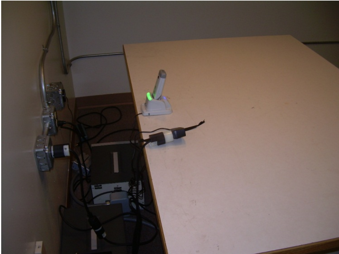
Photograph 9 – Back View Conducted Disturbance Worst Case Configuration
