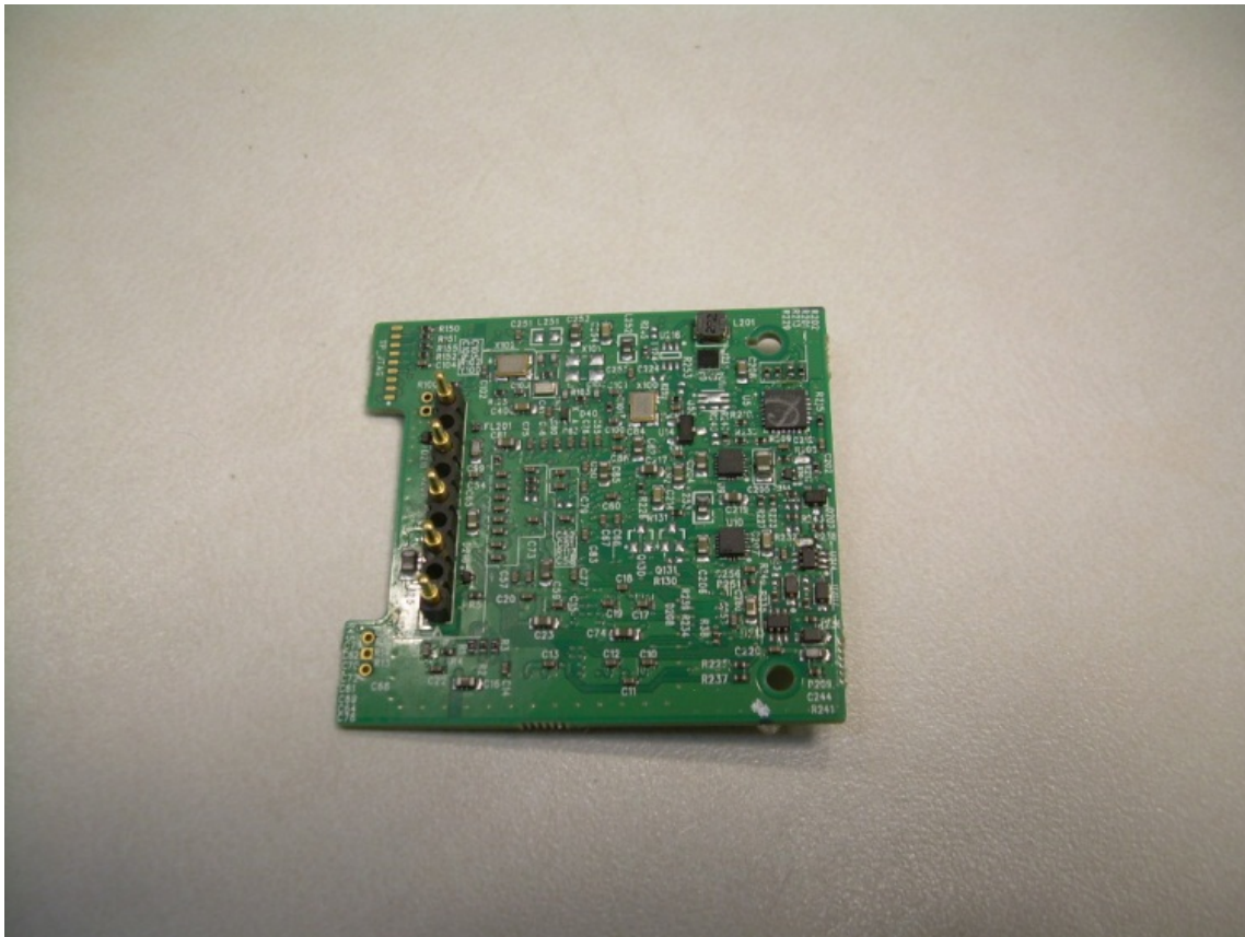
Photograph 21 – View of the Bottom Side of the Lower PCB
