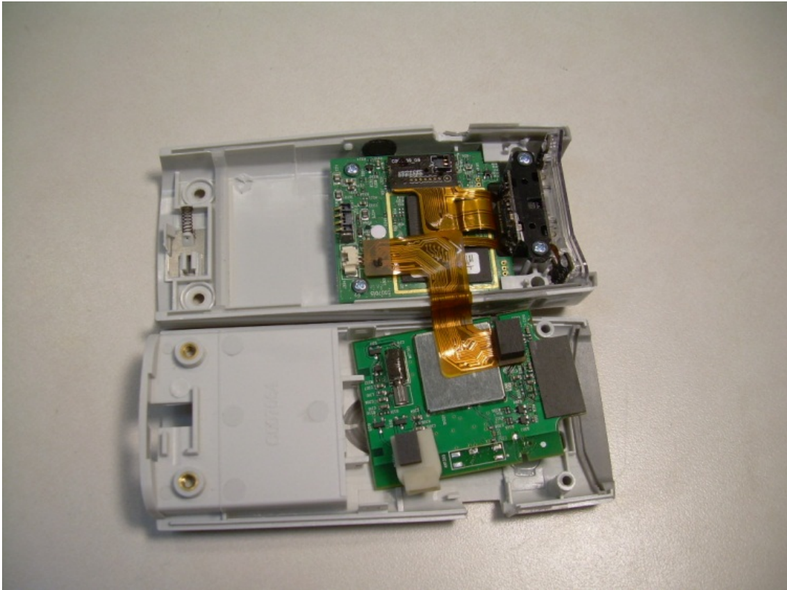
View with the Housing Opened Showing PCB Placement
