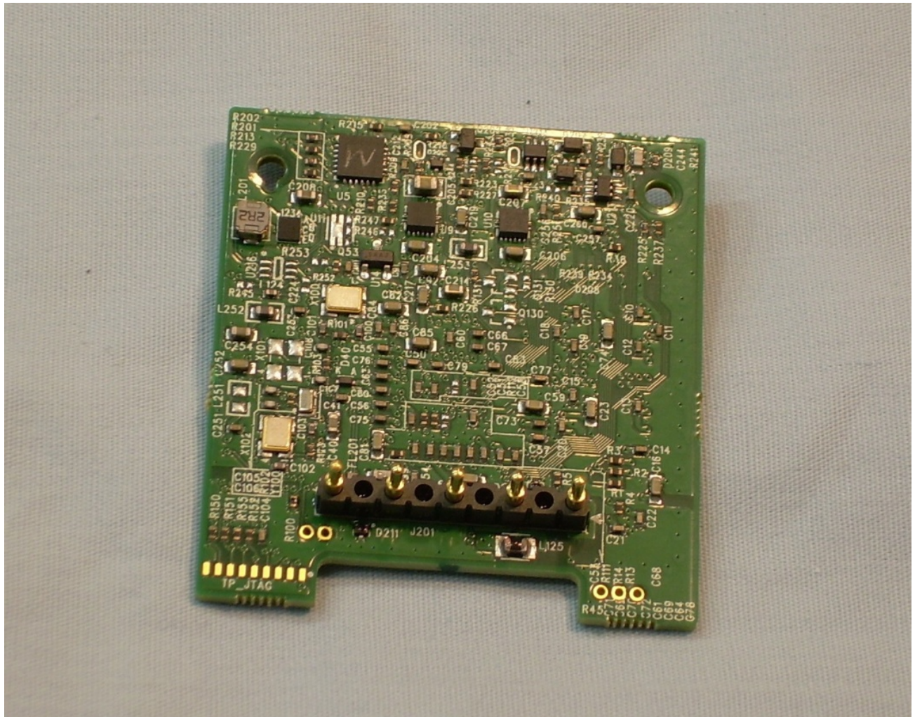
Photograph 21 – View of the Bottom Side of the Lower PCB
