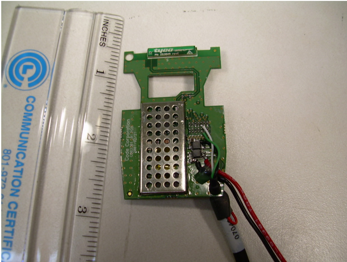
Component Side of PCB with RF Shield
