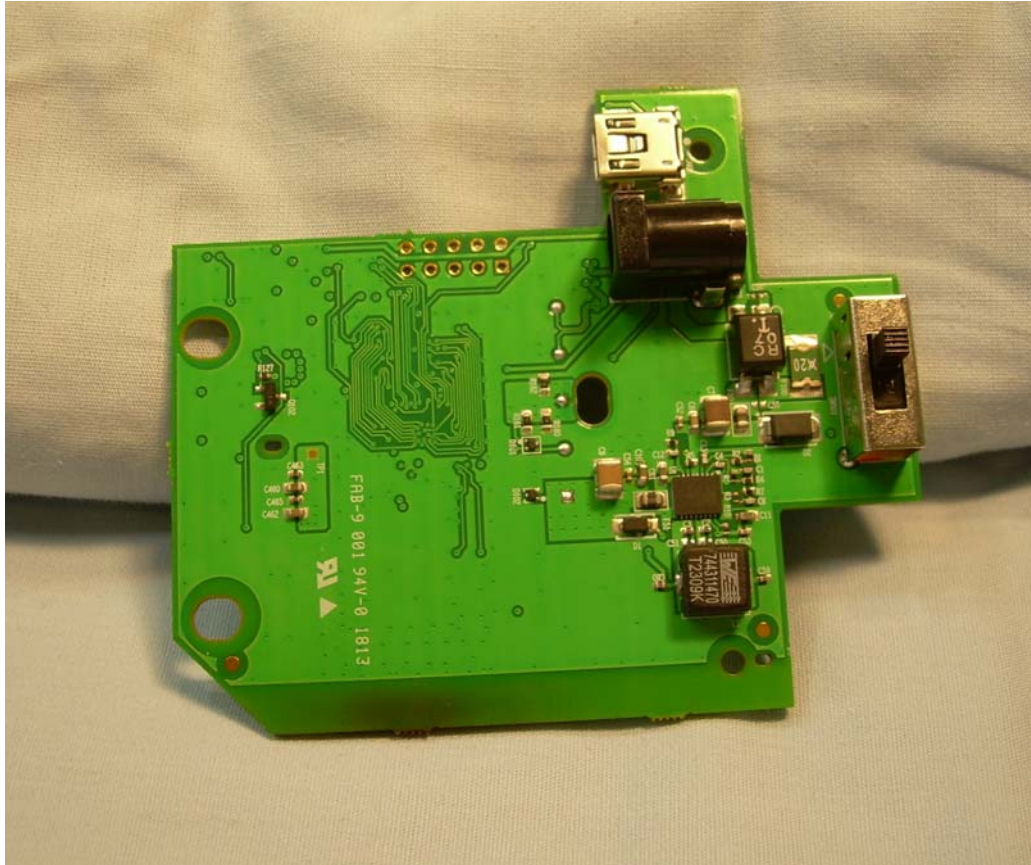
View of the Bottom Side of the PCB
