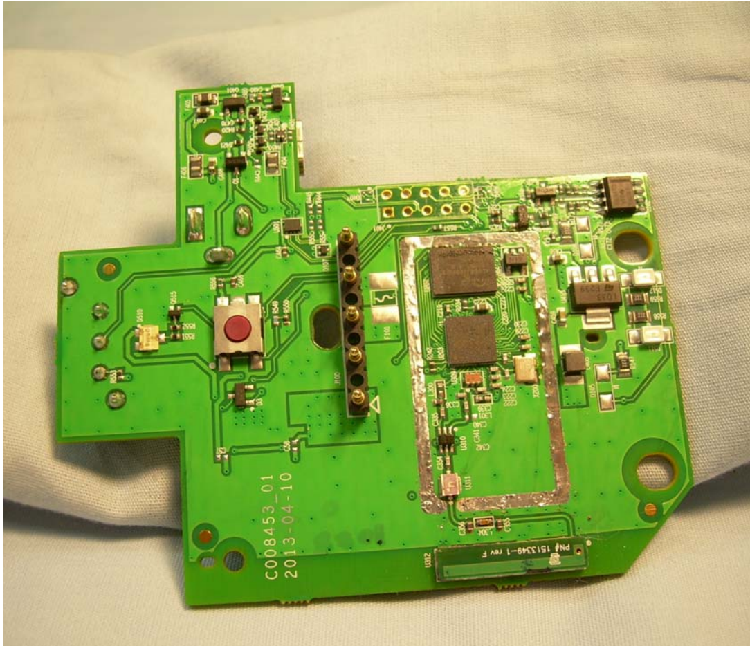
View of the Top Side of the PCB
