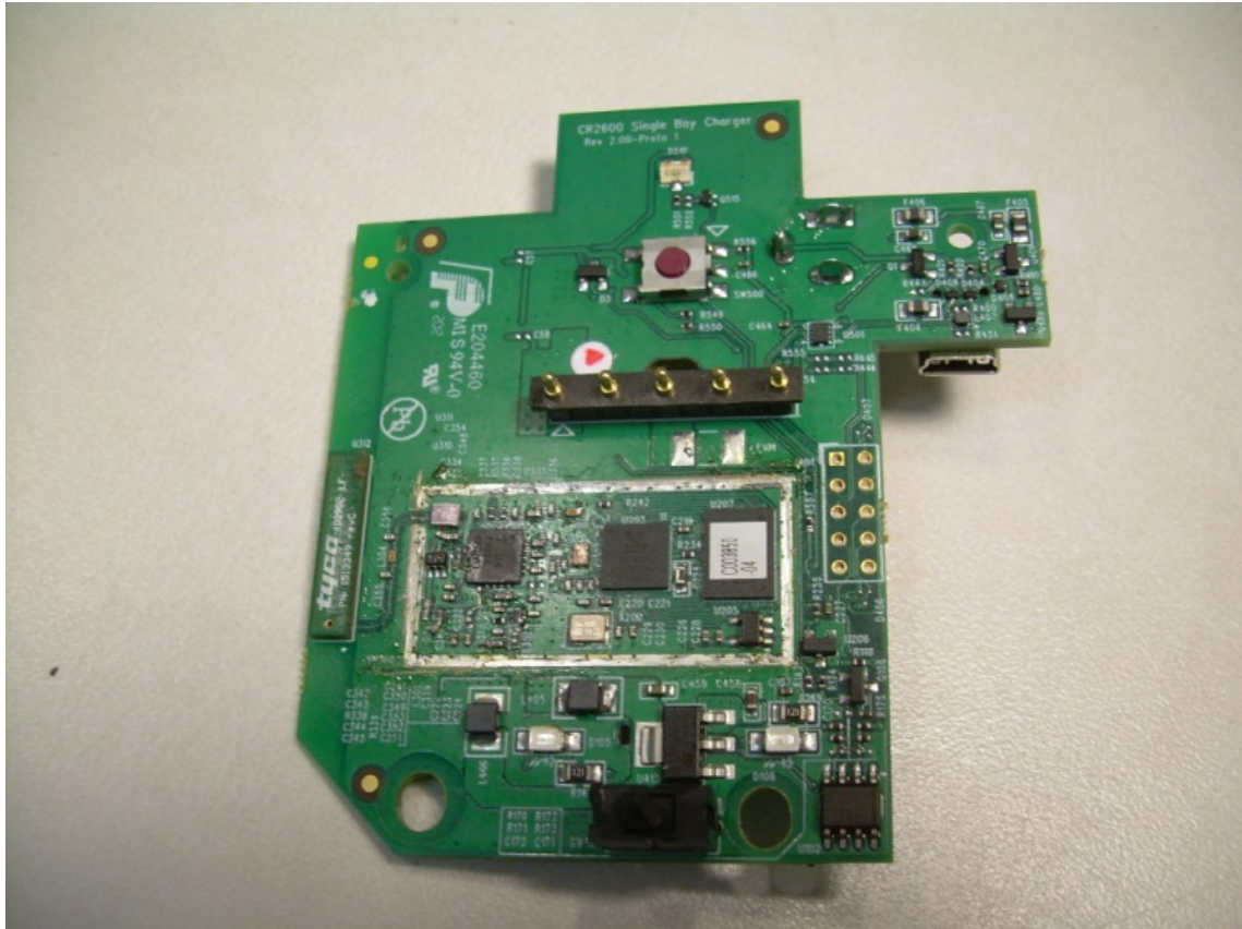
Photograph 10 – Top View of the PCB with RF Shield Removed
