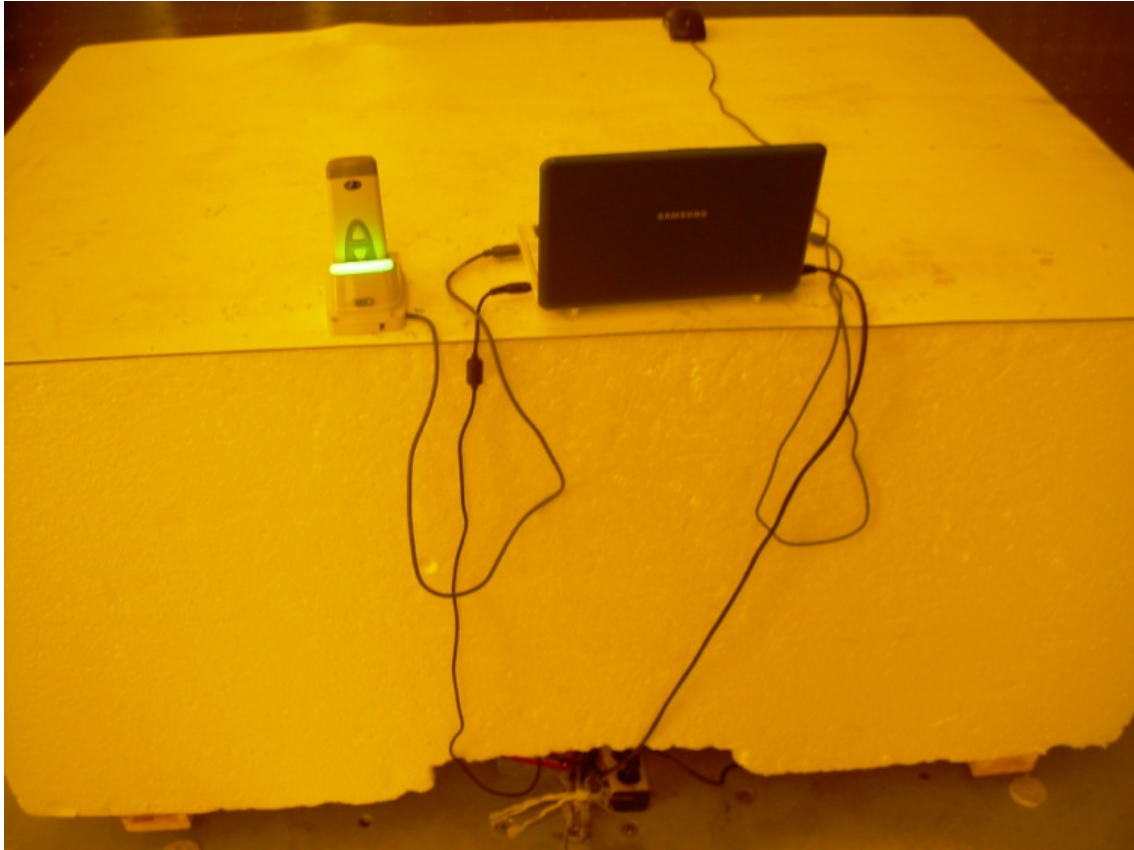
Photograph 2 – Back View Radiated Spurious Emission – USB Powered Configuration
