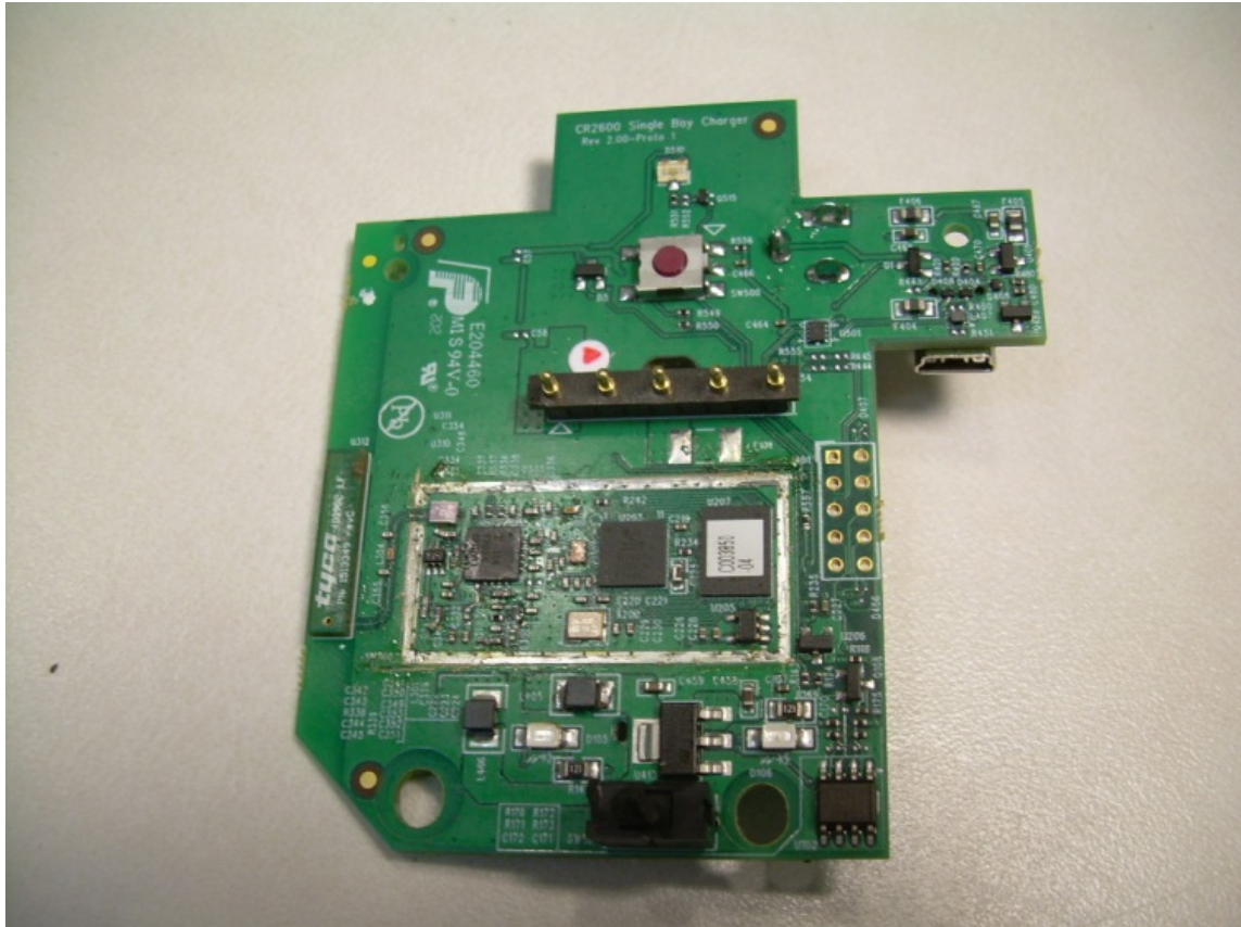
Top View of the PCB with RF Shield Removed
