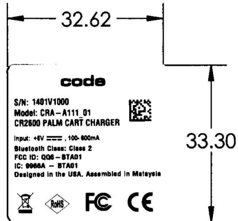
CRA-A111 Label Placement on Back
