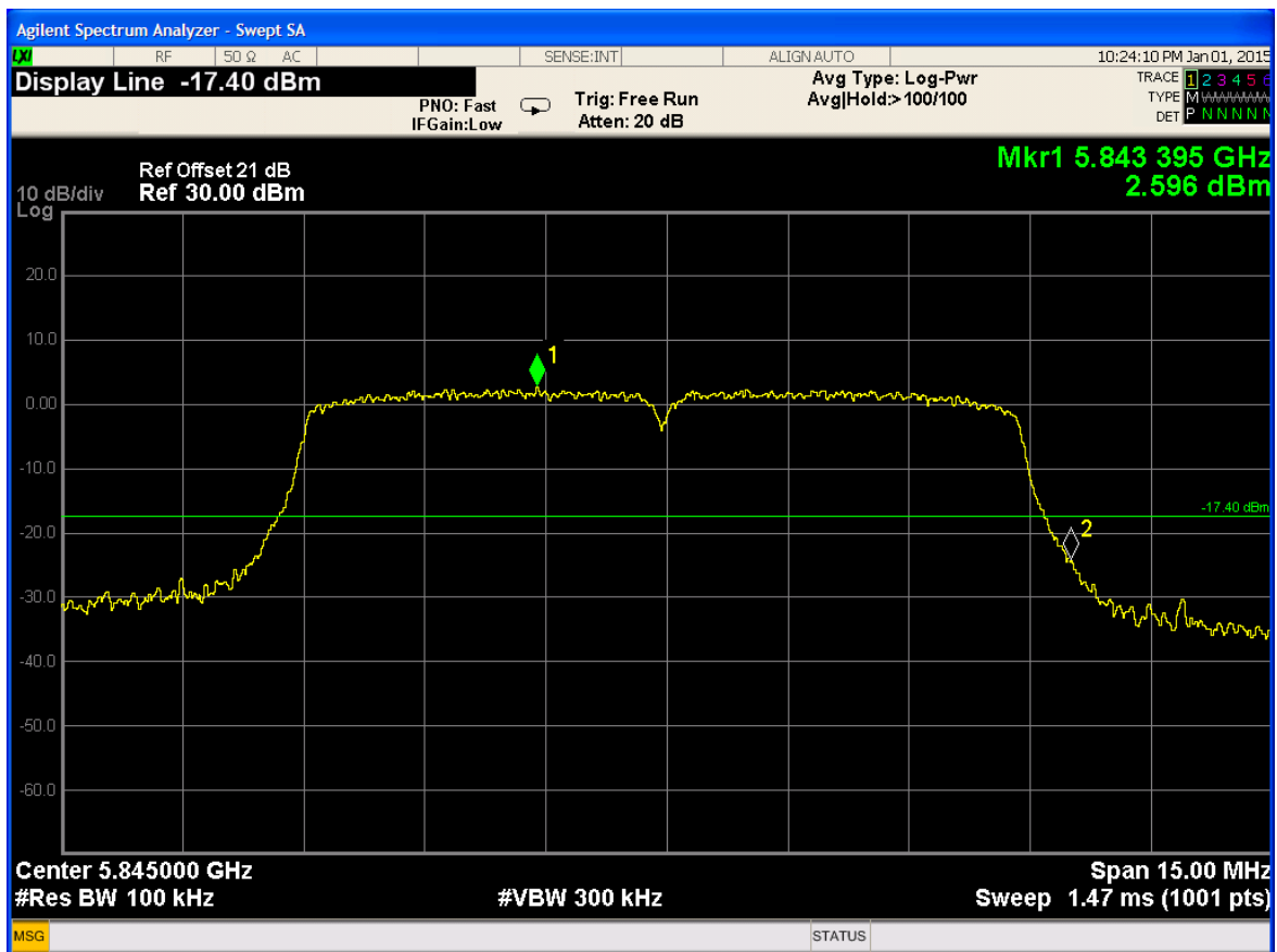
Plot Out of Band Conducted Emission/ 58
