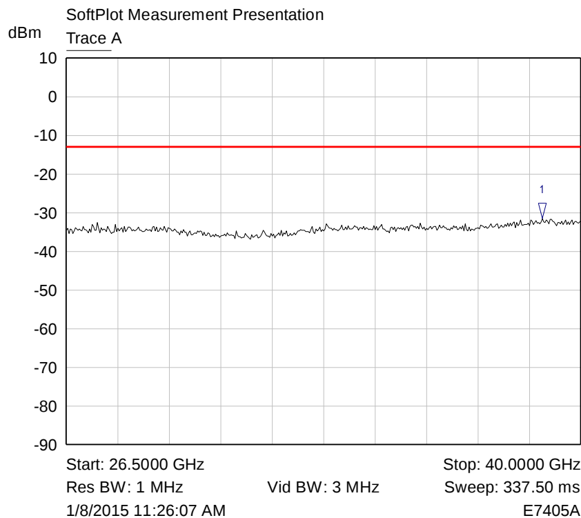
Plot Out of Band Conducted Emission/ 85
