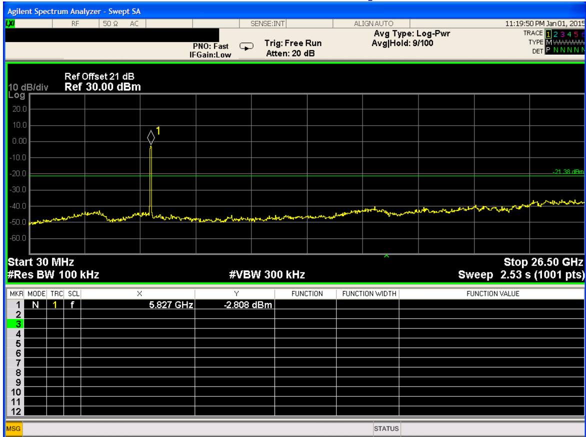
Plot Out of Band Conducted Emission/ 85
