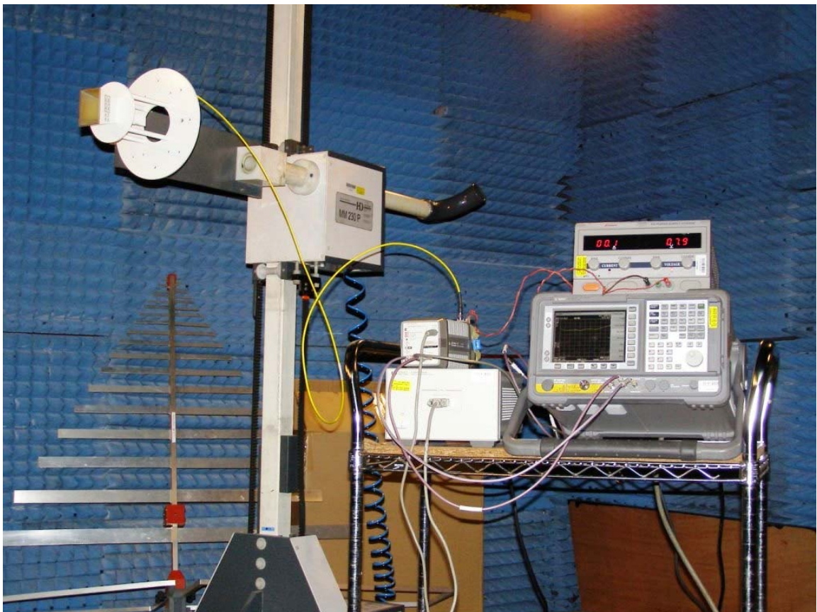
Radiated Emission Setup
